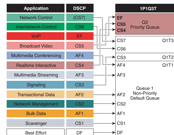
Figure 2 Catalyst 3560-X/3750-X Ingress Queuing Model
