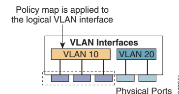
Figure 3 VLAN-Based QoS
