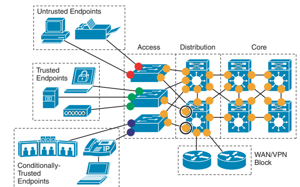
Figure 7 Medianet Campus Port QoS Roles
