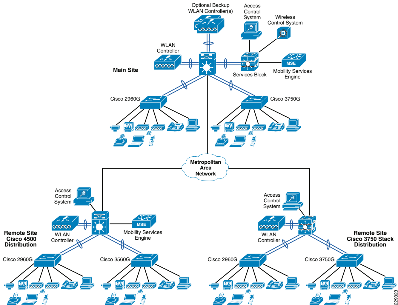
Figure 6-4 High-Level View of the SEDP With Hybrid Context-Aware Services
