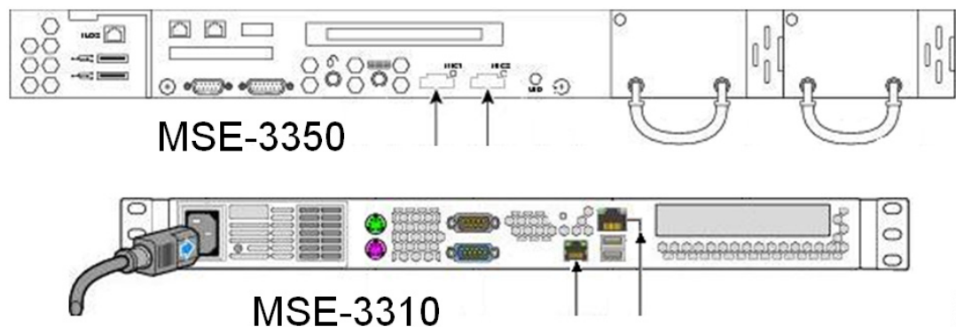
Figure 6-5 Rear Panel Illustration of MSE-3350
