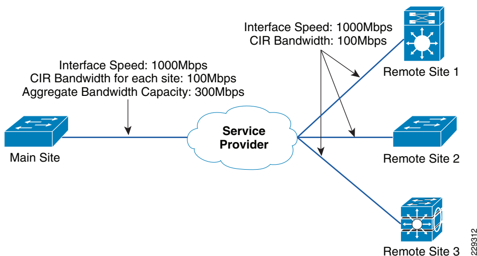
Figure 3-5 Bandwidth Capacity Planning for Three Remote Sites
