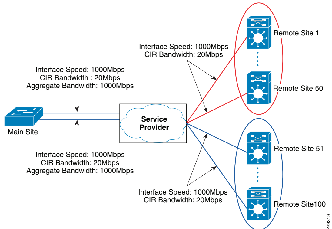
Figure 3-6 Bandwidth Capacity Planning for 100 Remote Sites
