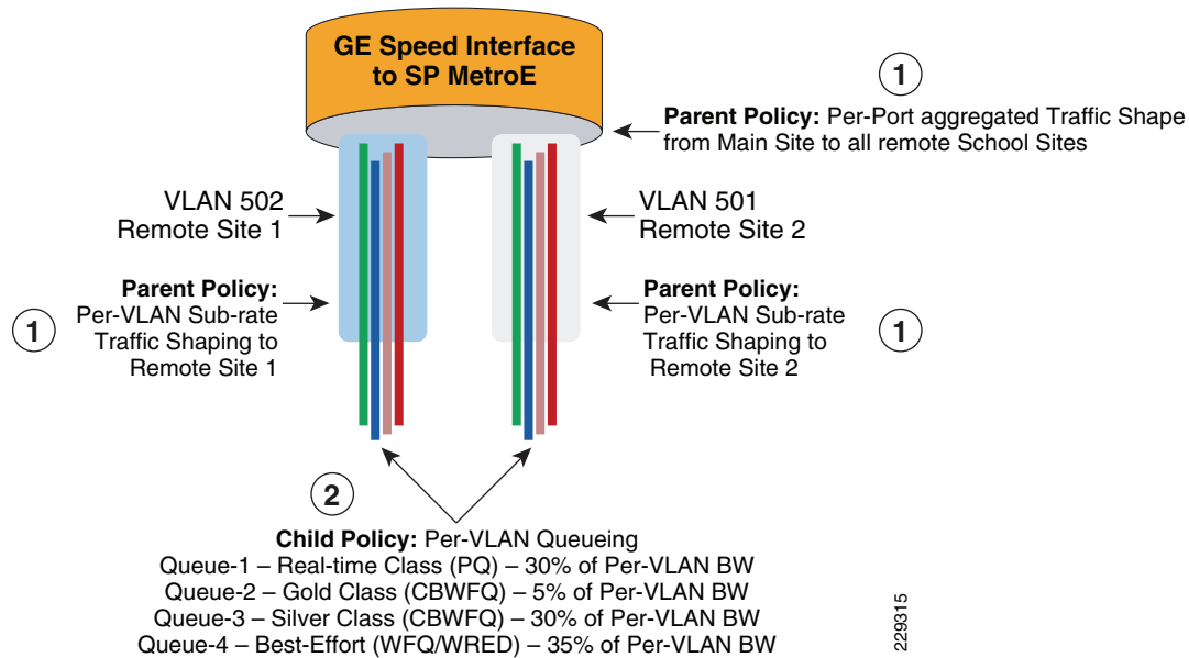
Figure 3-8 Hierarchical Policy Implementation at Main Office
