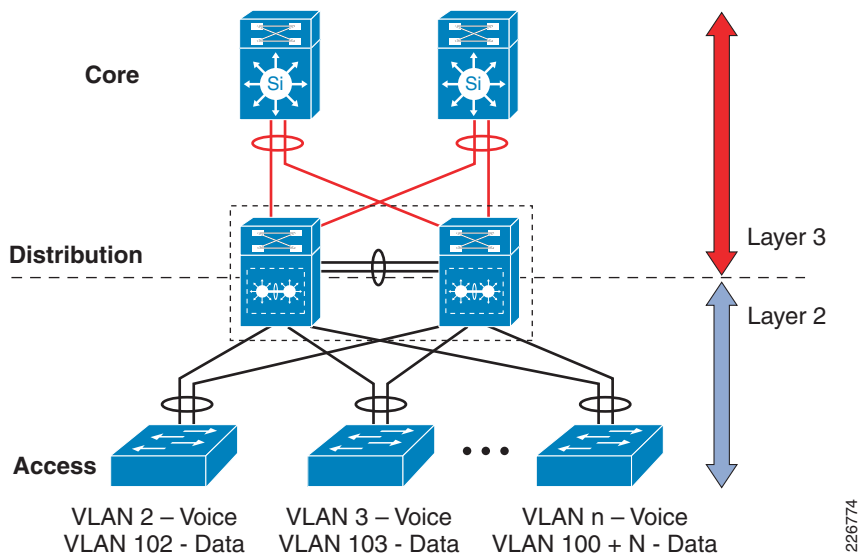
Figure 5-3 VSS Design
