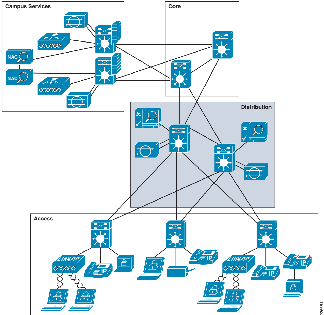
Figure 5-6 Campus Distribution Layer
