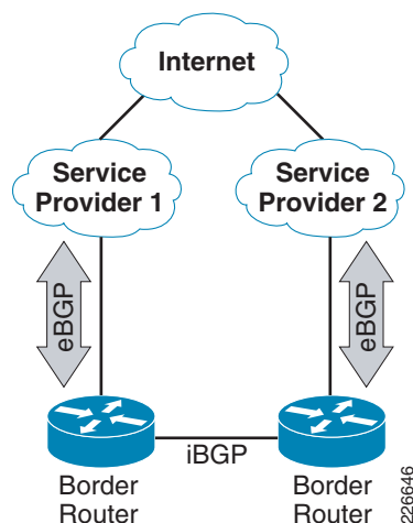
Figure 6-23 BGP Design
