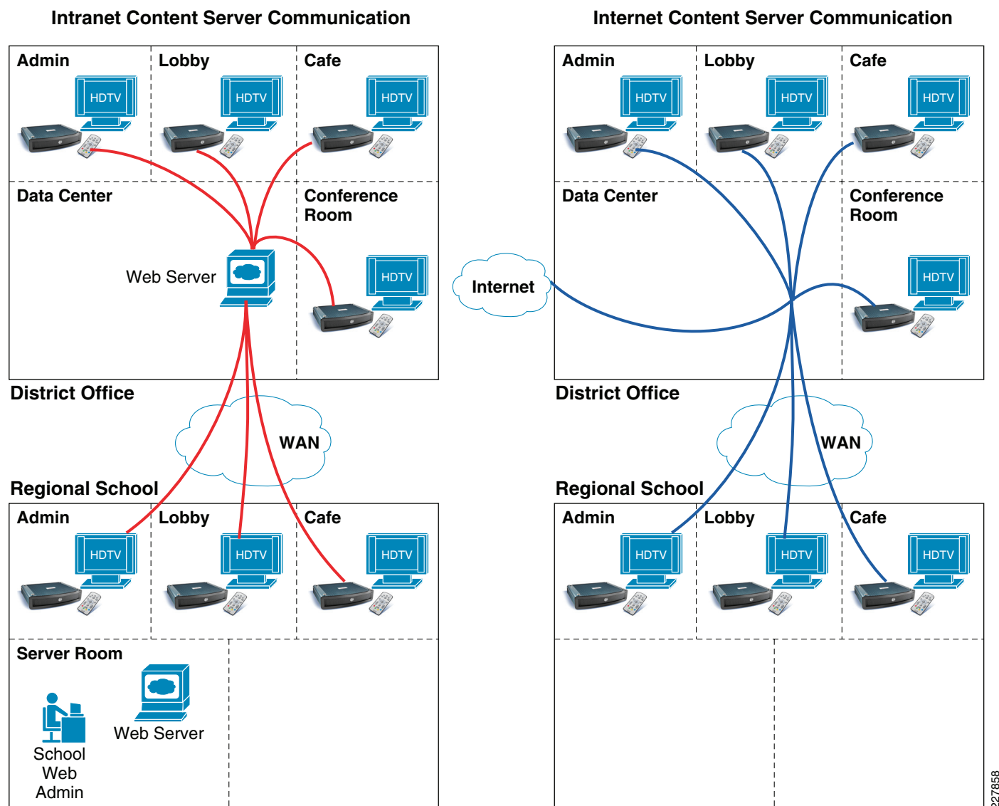
Figure 8-11 Distributed Content Server Communication
