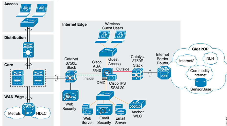
Figure 22 Internet Edge Firewall
