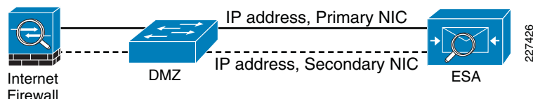
Figure 9 Cisco IronPort ESA NIC Pairing
