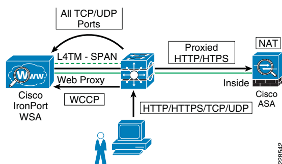
Figure 12 L4TM Deployment
