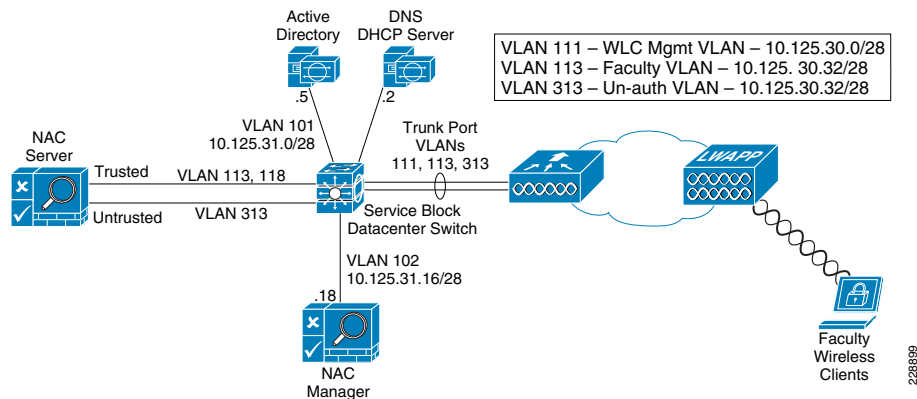
Figure 58 Layer-2 OOB NAC Deployment Topology for Faculty Wireless Clients
