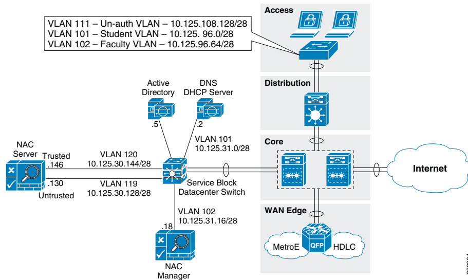
Figure 43 NAC L3 OOB Logical Topology Diagram
