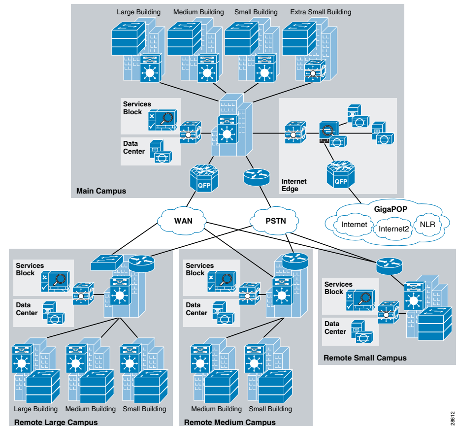
Figure 2 Community College Reference Design Overview
