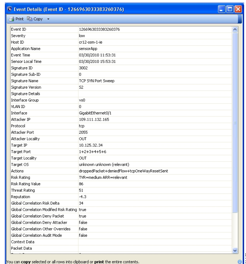
Figure 30 Detail View of a TCP SYN Port Sweep from an Attacker with a Negative Reputation Score
