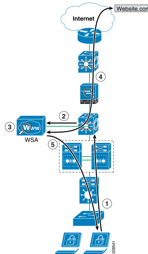
Figure 11 WCCP Redirection
