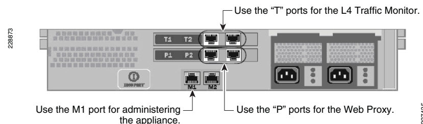
Figure 32 WSA Interfaces
