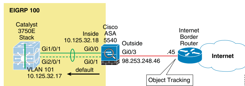
Figure 24 Cisco ASA Static Route
