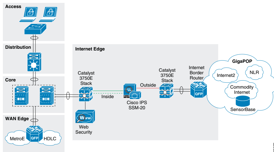
Figure 31 WSA Deployment
