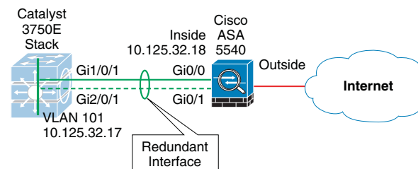
Figure 23 Cisco ASA Redundant Interface
