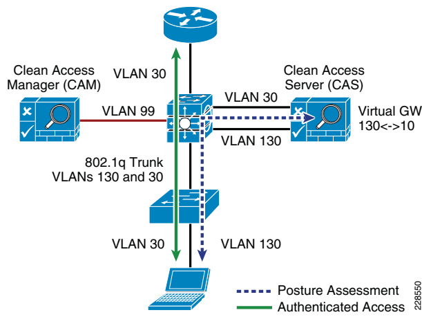
Figure 21 Layer 2 OOB Topology
