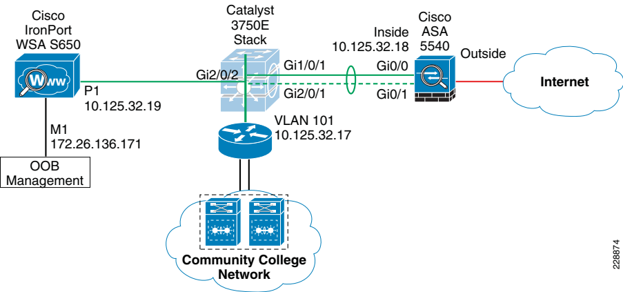
Figure 33 WSA Network Topology
