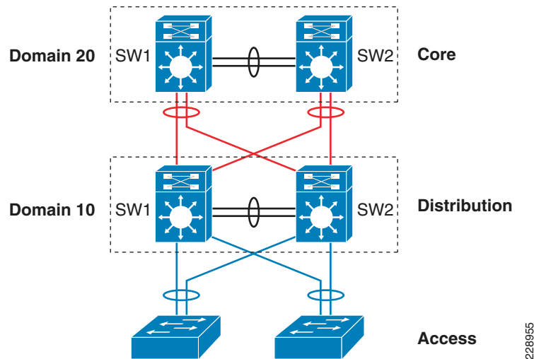
Figure 3-25 VSS Domain and Switch ID
