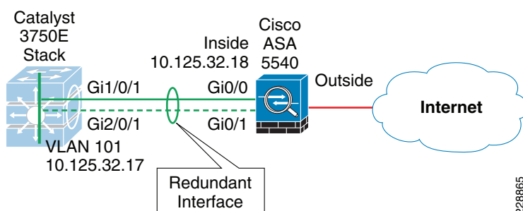
Figure 6-23 Cisco ASA Redundant Interface
