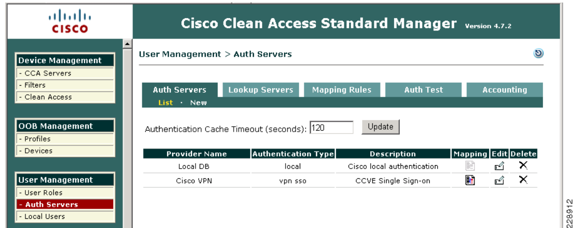
Figure 6-71 Role Mapping
