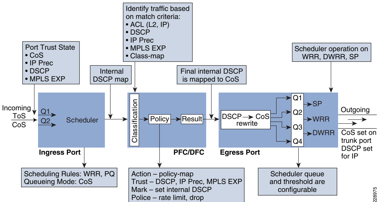
Figure 3-51 Cisco Catalyst 6500-E PFC QoS Architecture
