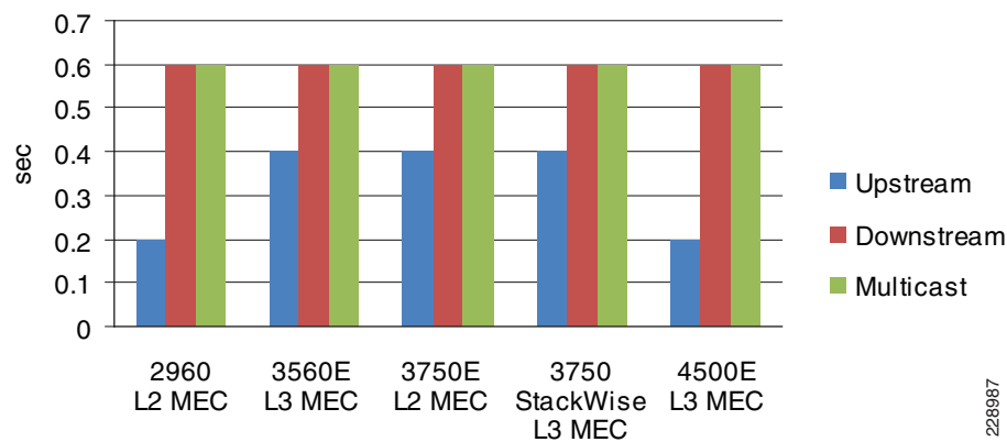
Figure 3-67 Catalyst 6500-E VSS Inter-Chassis MEC Link Recovery Analysis
