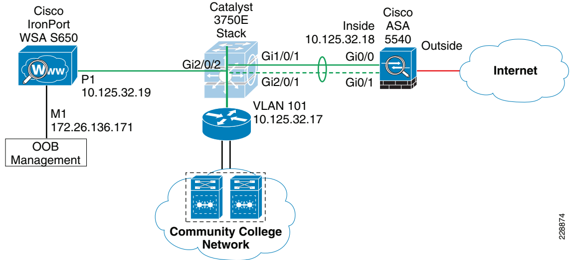
Figure 6-33 WSA Network Topology
