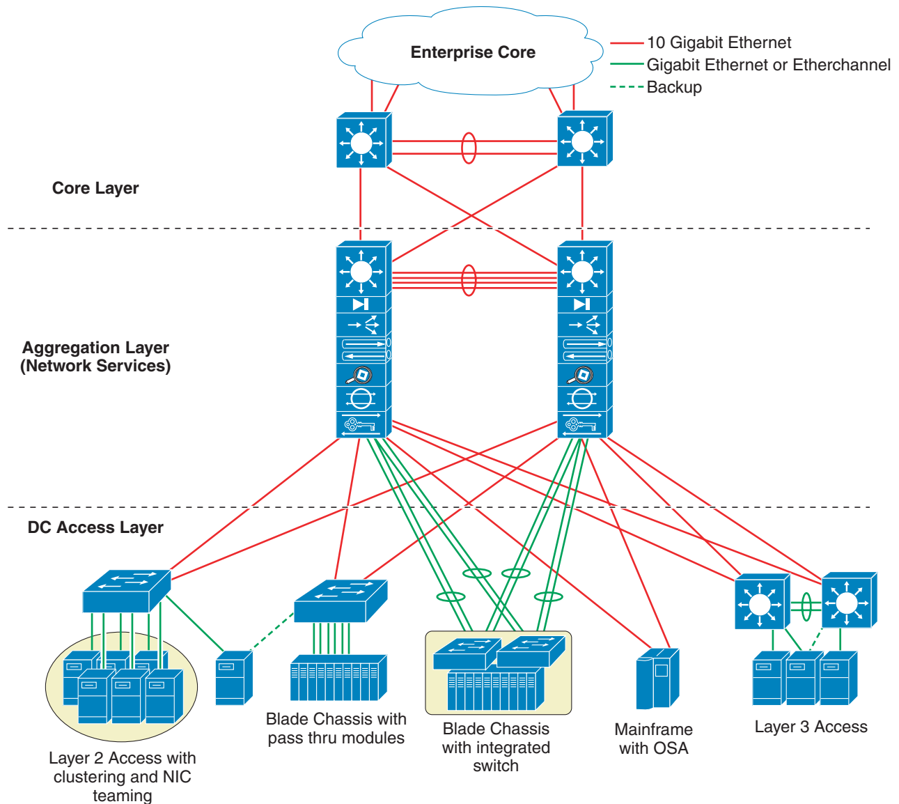
Figure 32 Cisco Data Center Architecture
