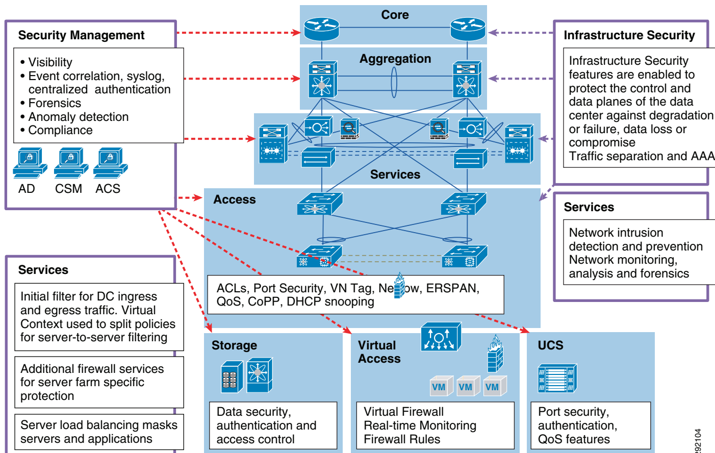
Figure 5 Security Framework of the Cisco VMDC Architecture
