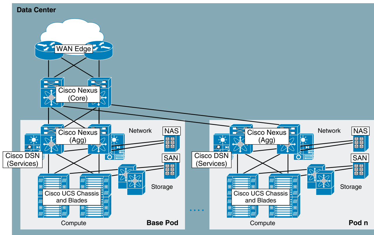
Figure 3 Scalable Data Center Design Using Modular Building Blocks
