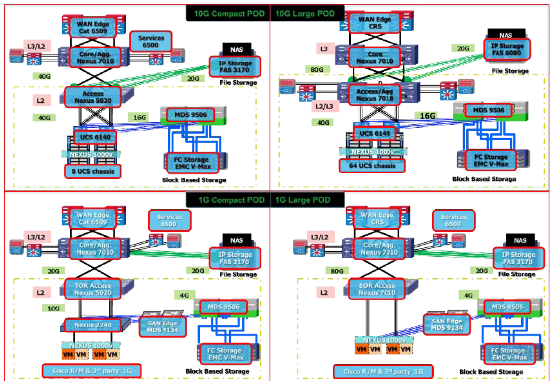
Figure 1-10 VMDc 2.X Topology Options
