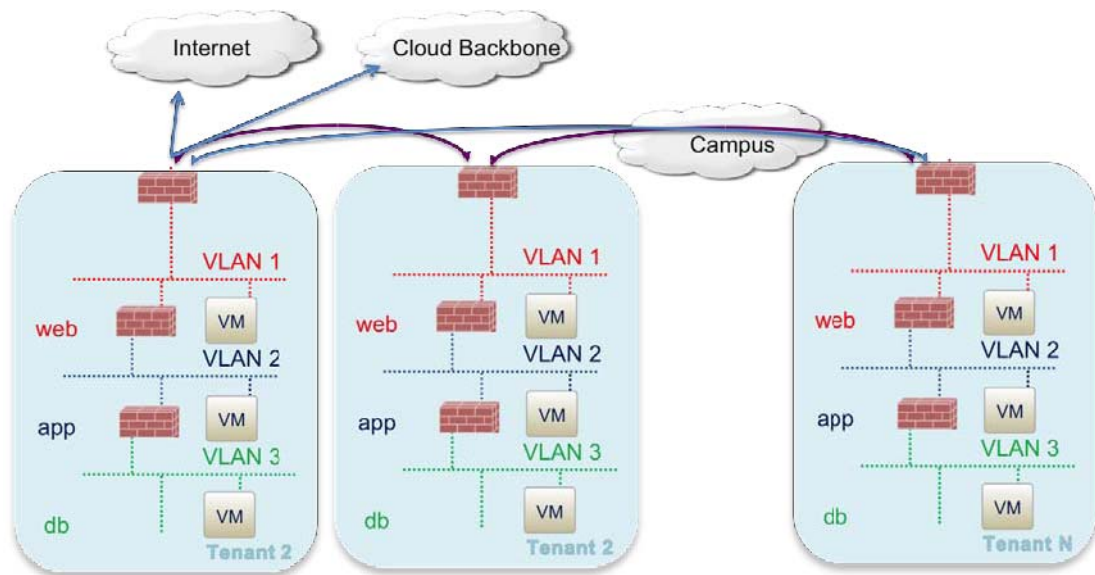
Figure 2-2 Three-Tier Firewall
