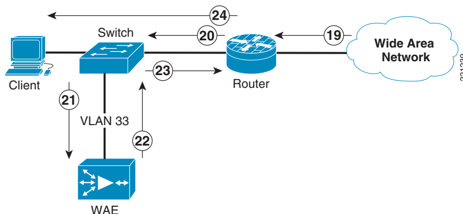
Figure 17 Traffic Pattern—Extended Service Branch Return Flow Example
