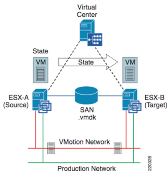
Figure 2-14 vMotion Process
