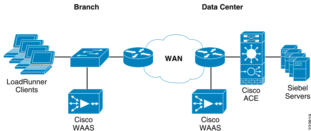
Figure 10 Testing Scenario
