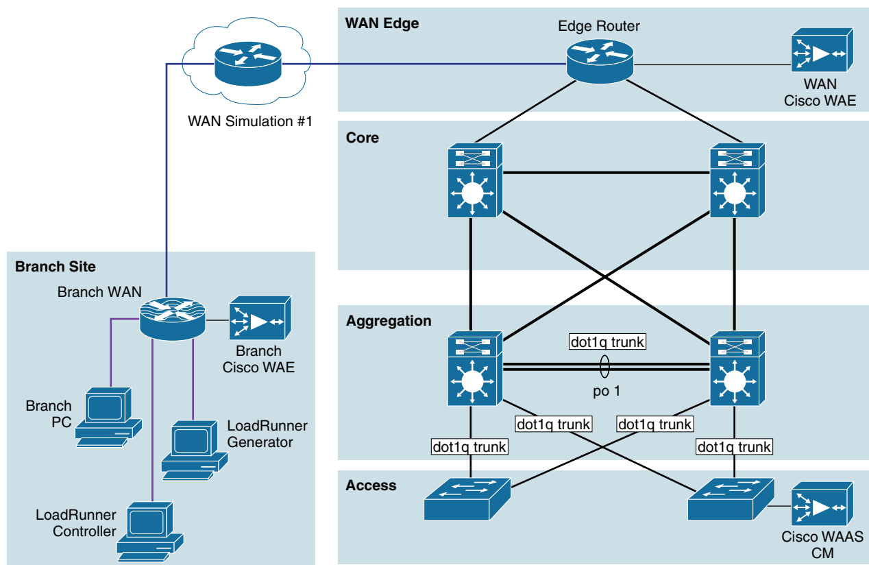
Figure 8 Network Topology
