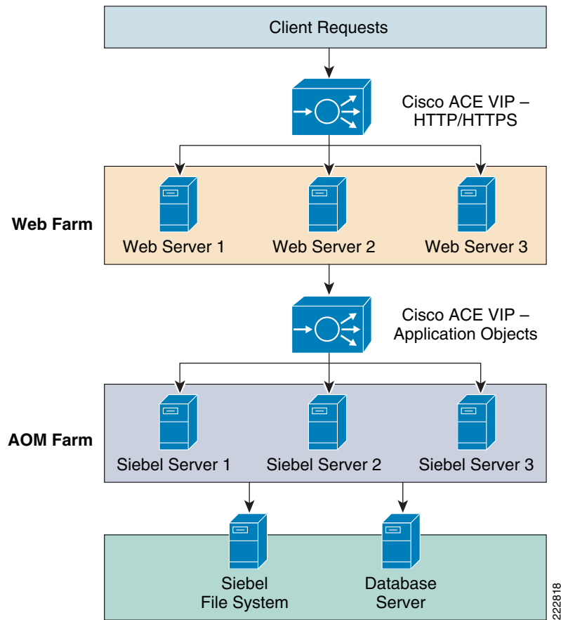
Figure 7 Network Topology
