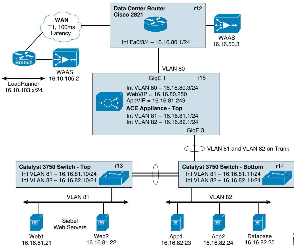
Figure 17 Cisco ACE Appliance Configuration
