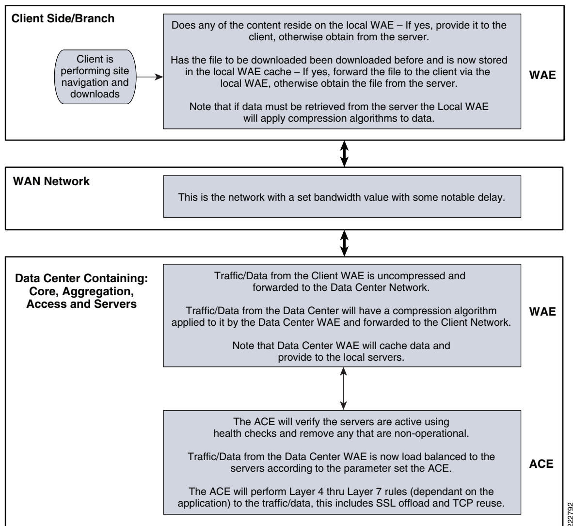
Figure 2 Process Flow
