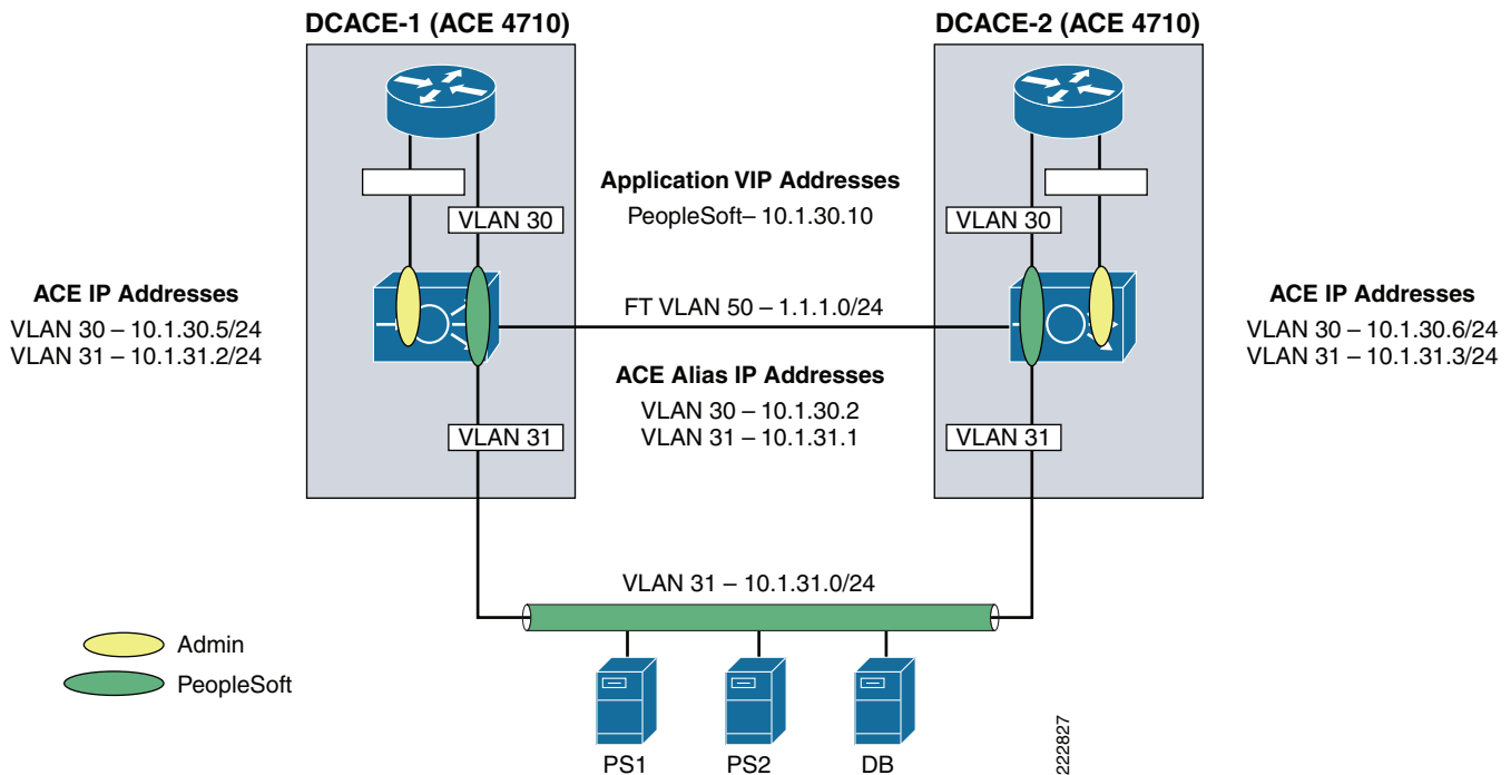
Figure 6 Network Topology
