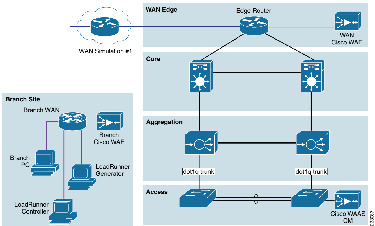
Figure 7 Network Topology
