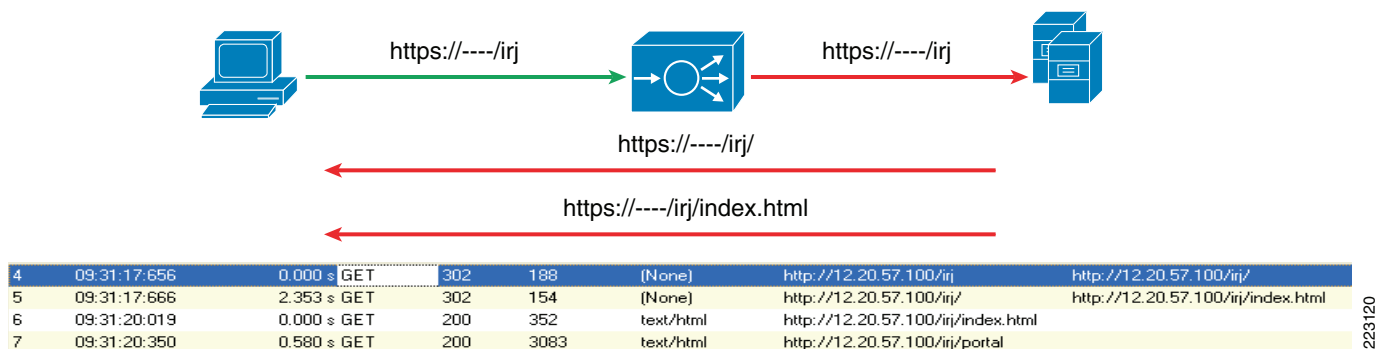
Figure 13 HTTP Redirects with SSL Offload
