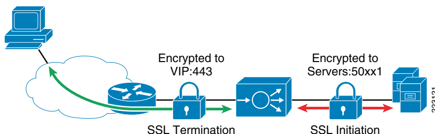
Figure 15 SSL Offload with Backend Encryption
