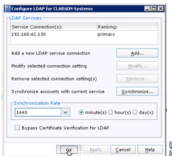
Figure 5-95 Adding LDAP Service
