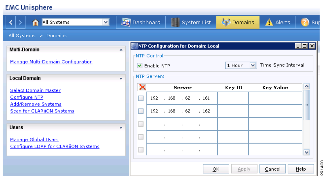
Figure 5-100 NTP Configuration for Domain: Local
