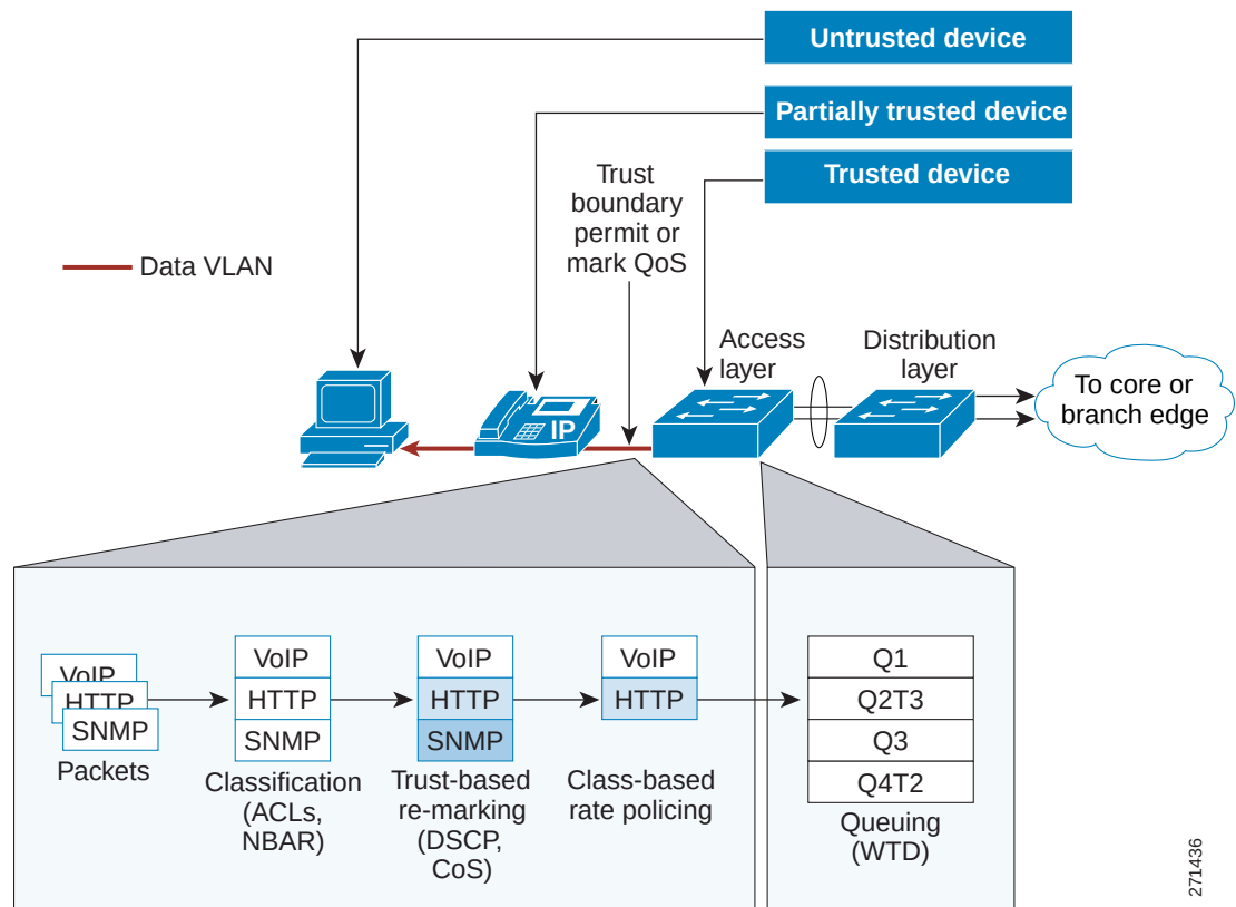
Figure 31 LAN Switch
