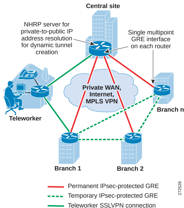
Figure 35 DMVPN mGRE architecture
