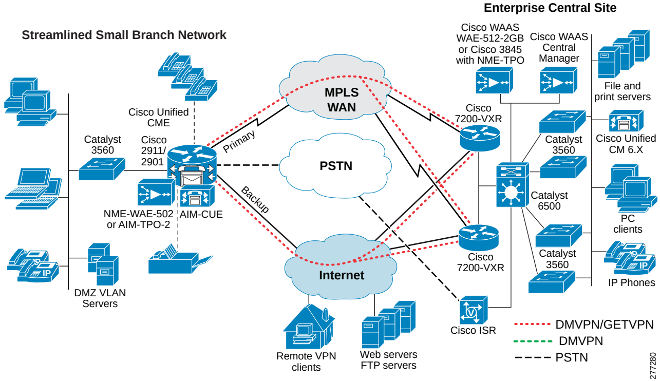
Figure 3 MPLS WAN, Cisco Unified CME Mode
