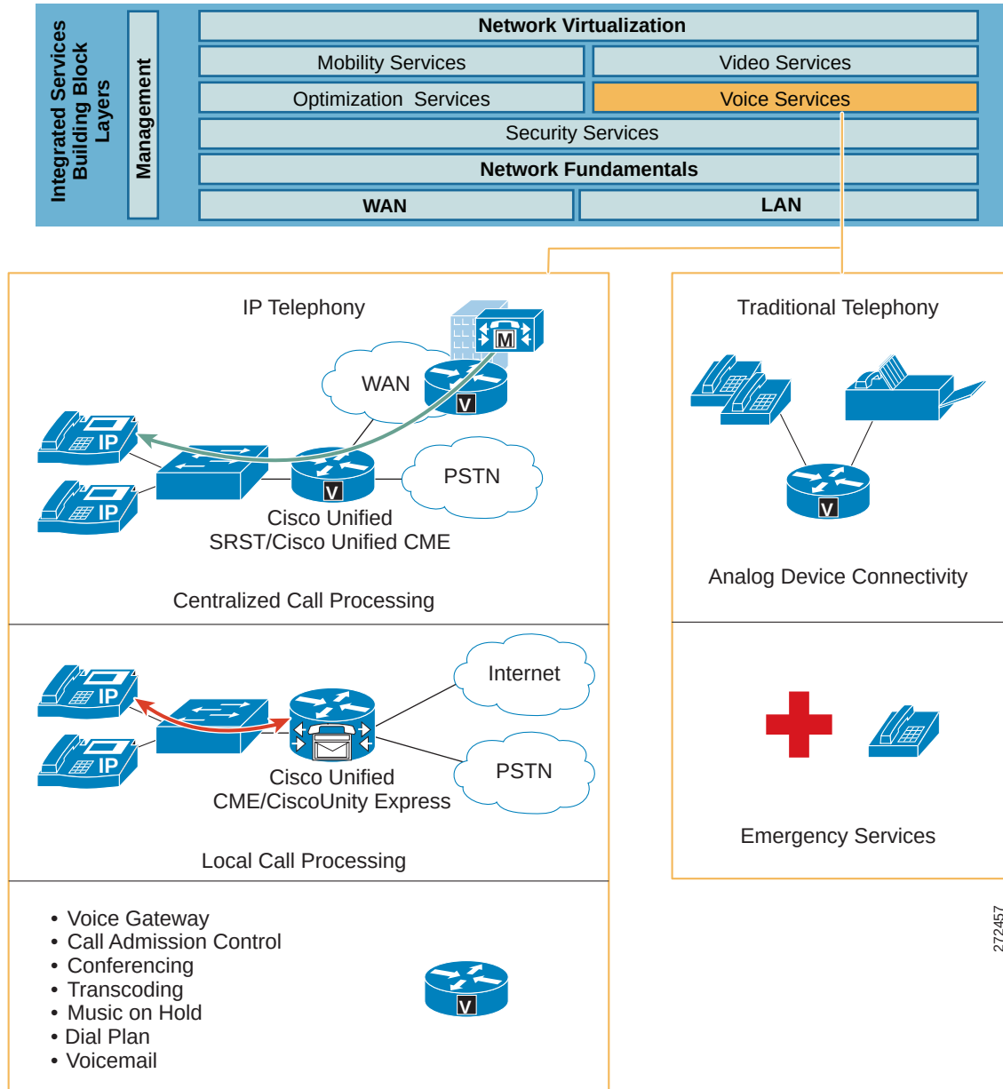
Figure 42 Voice Services
