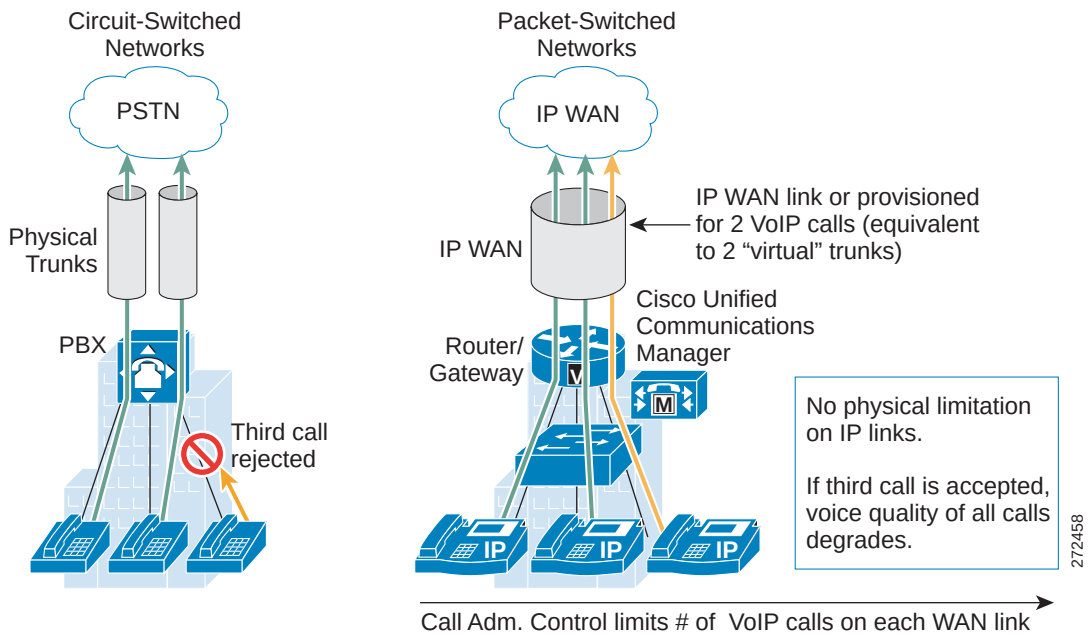
Figure 51 Traditional Versus VoIP Call Admission Control
