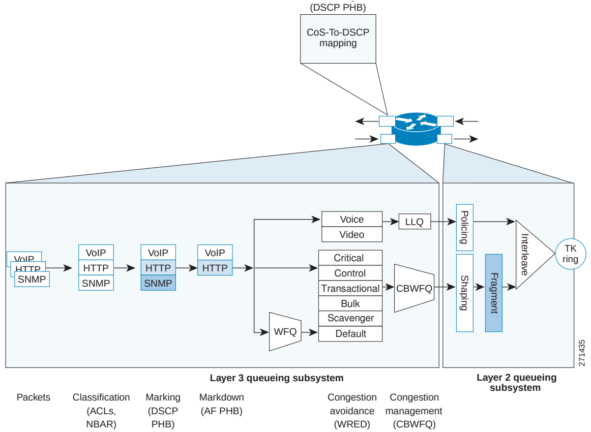
Figure 30 WAN Router
