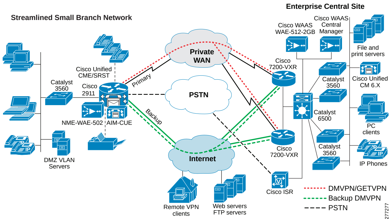
Figure 1 Streamlined Small Branch Network Test Bed
