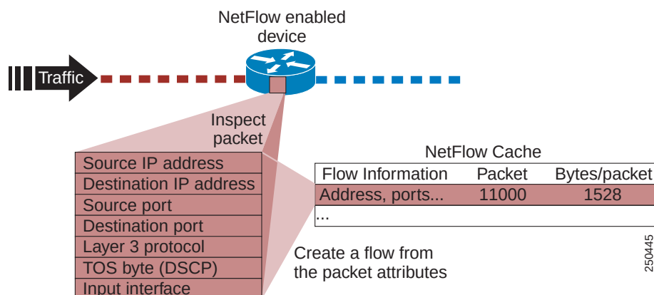
Figure 40 Data Captured by NetFlow
