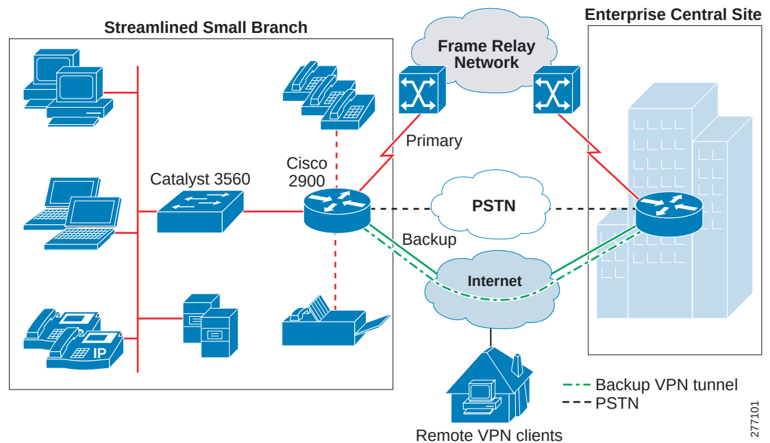
Figure 16 Streamlined Small Branch Network Frame Relay Service Deployment
