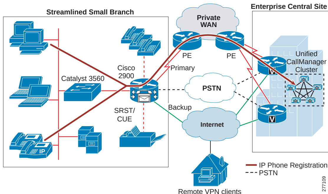
Figure 45 Centralized Call Control Model
