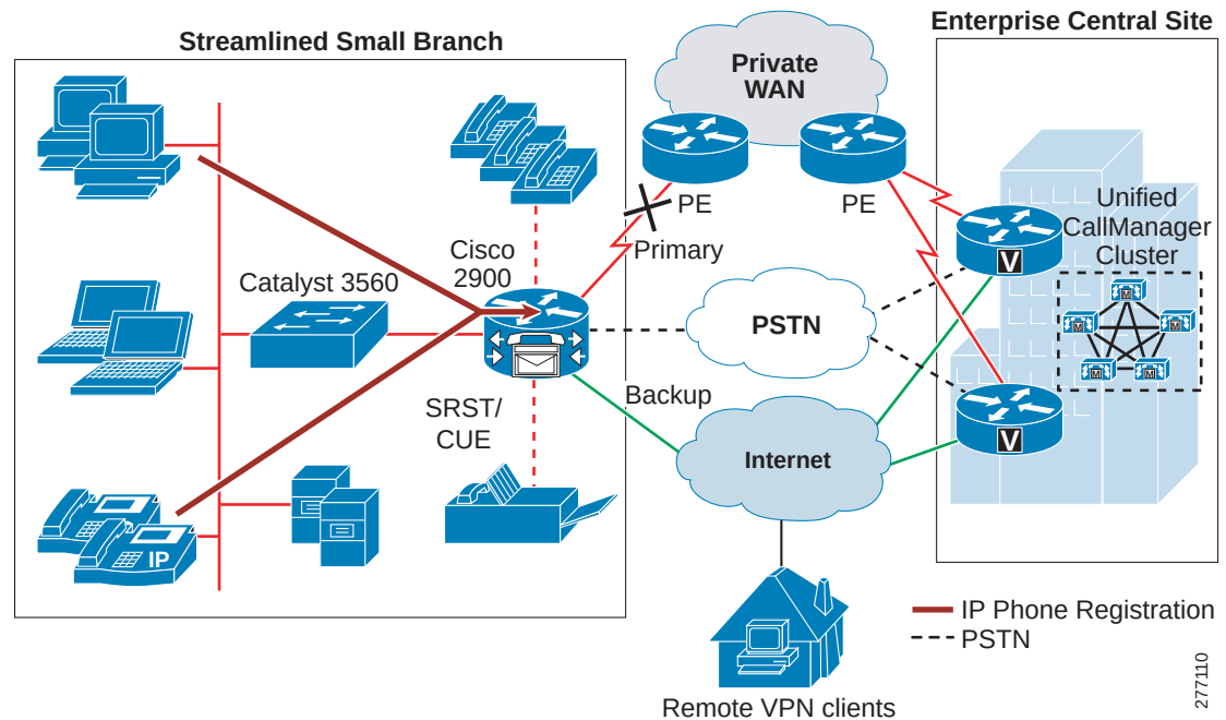
Figure 46 Cisco Unified SRST Mode for Centralized Call Control Model
