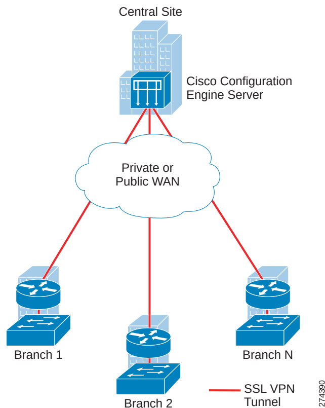
Figure 41 Deployment of CCE in the Streamlined Small Branch Network.
