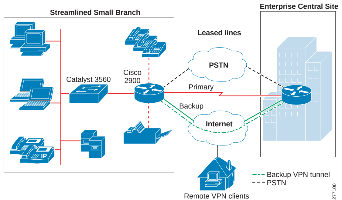
Figure 15 Streamlined Small Branch Network Leased Line Deployment
