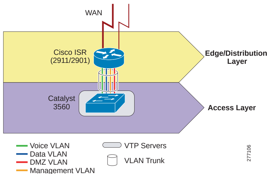
Figure 23 VLAN Trunks and VTP Configuration
