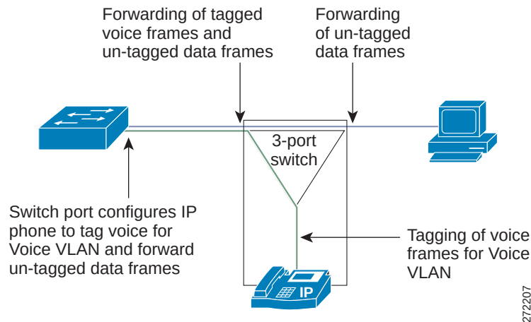
Figure 22 Integrated Switch in Cisco Unified IP Phone 7900 Series
