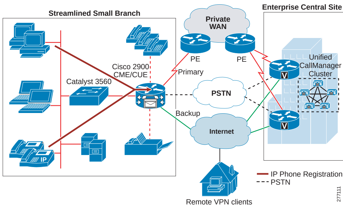
Figure 47 Distributed Call Control Model
