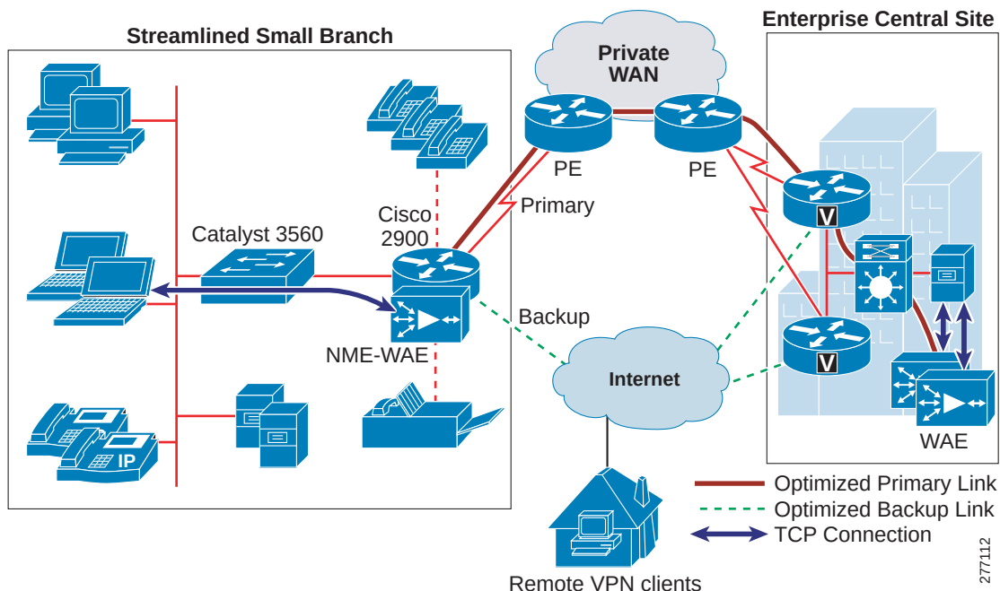
Figure 57 Cisco WAAS Optimization Path
