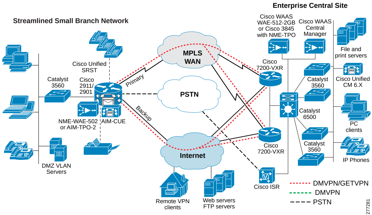
Figure 4 MPLS WAN, Cisco Unified SRST Mode
