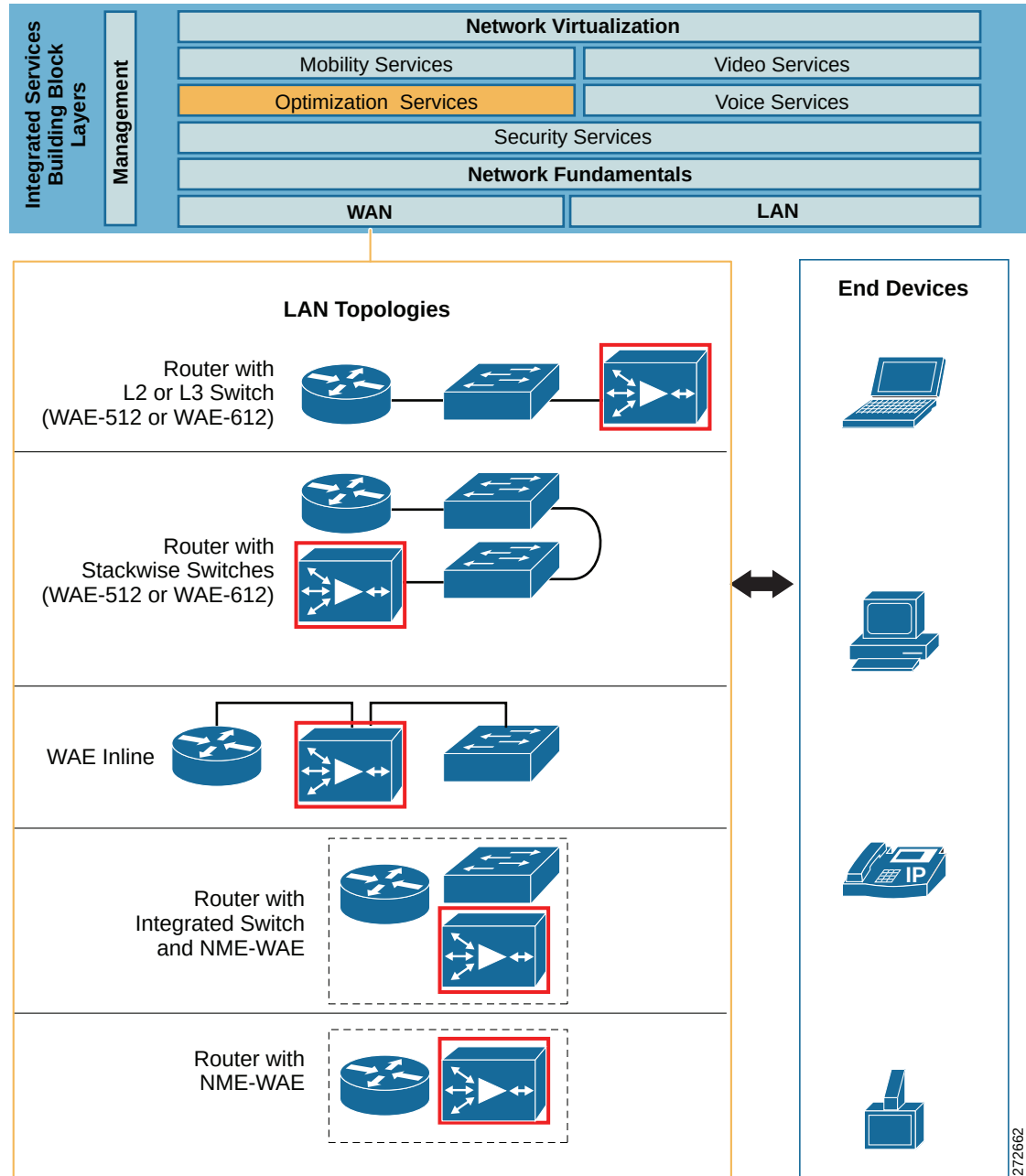
Figure 55 Cisco WAAS Deployment Options
