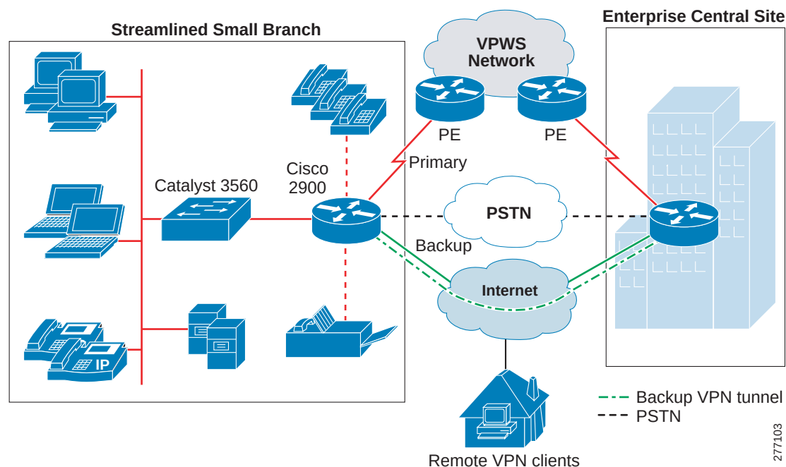
Figure 18 The Streamlined Small Branch Network VPWS Deployment
