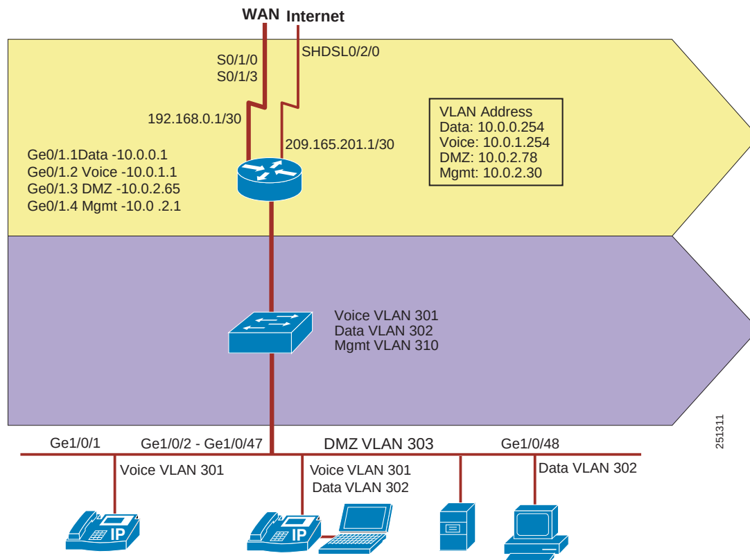
Figure 28 Sample Address Assignment for the Streamlined Small Branch Network
