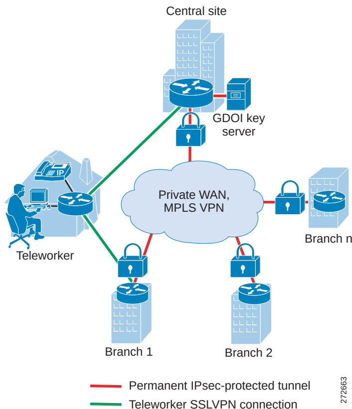
Figure 36 Any-to-Any GETVPN connectivity
