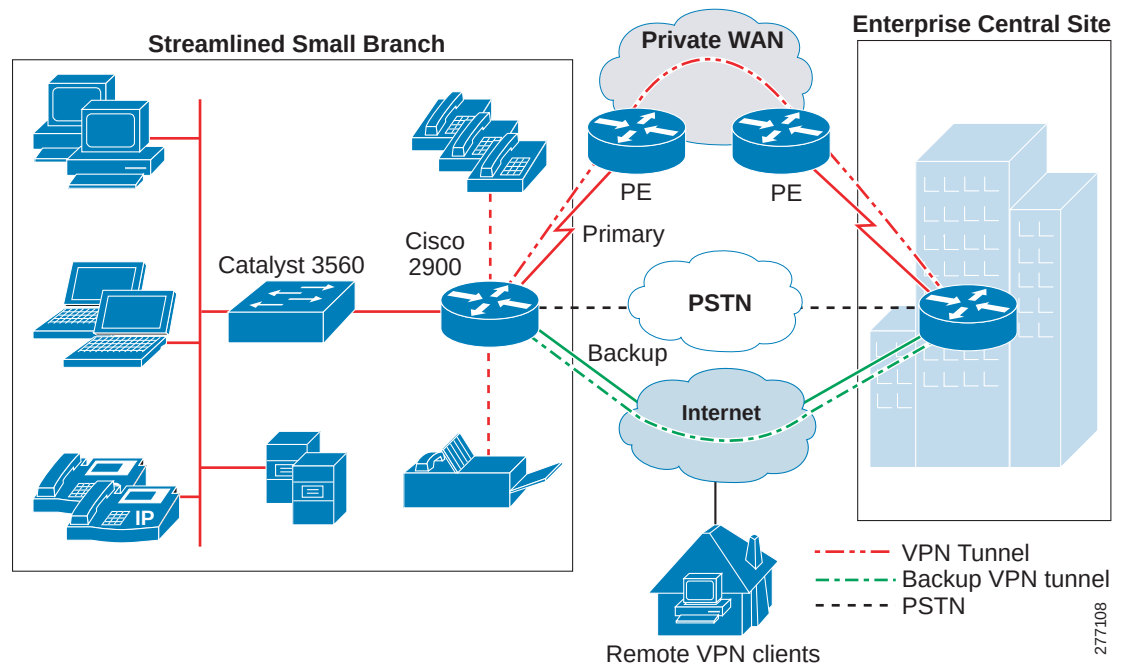
Figure 34 The Streamlined Small Branch Network Private WAN Deployment
