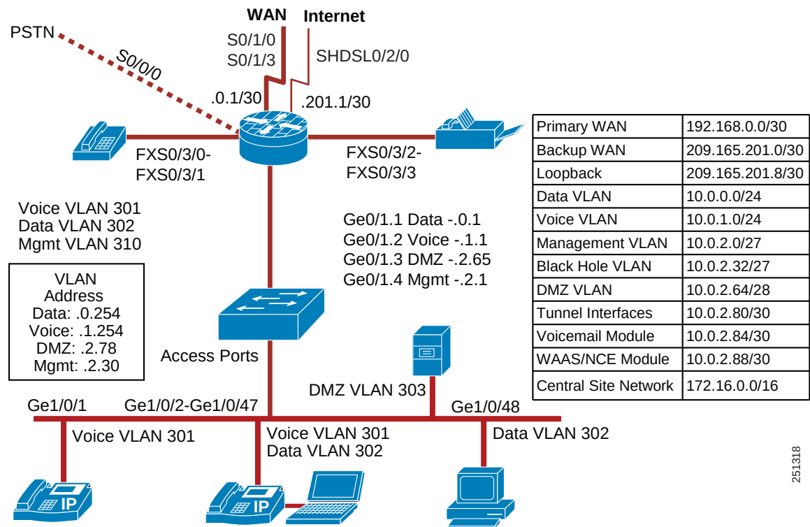
Figure 2 Streamlined Small Branch Network Topology
