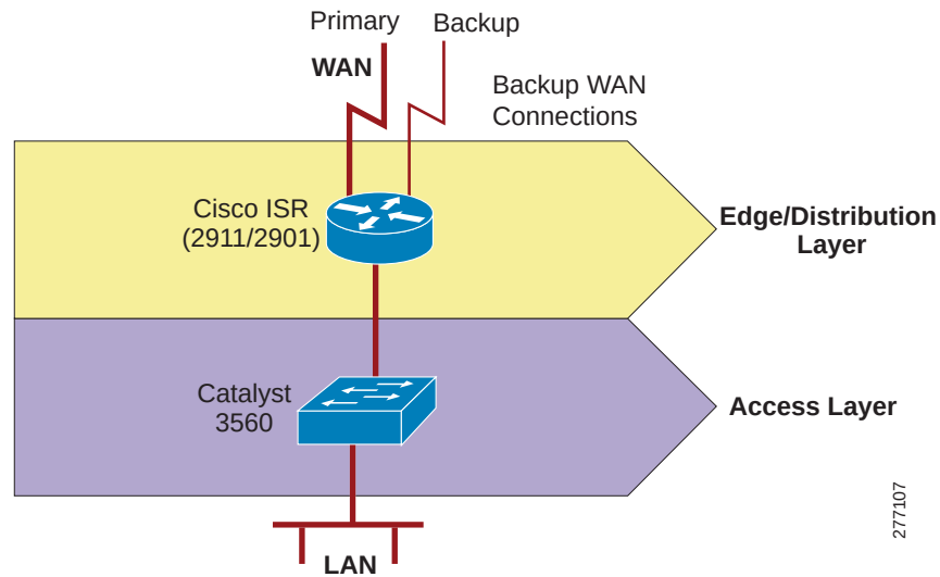
Figure 25 High Availability and Rapid Recovery Components
