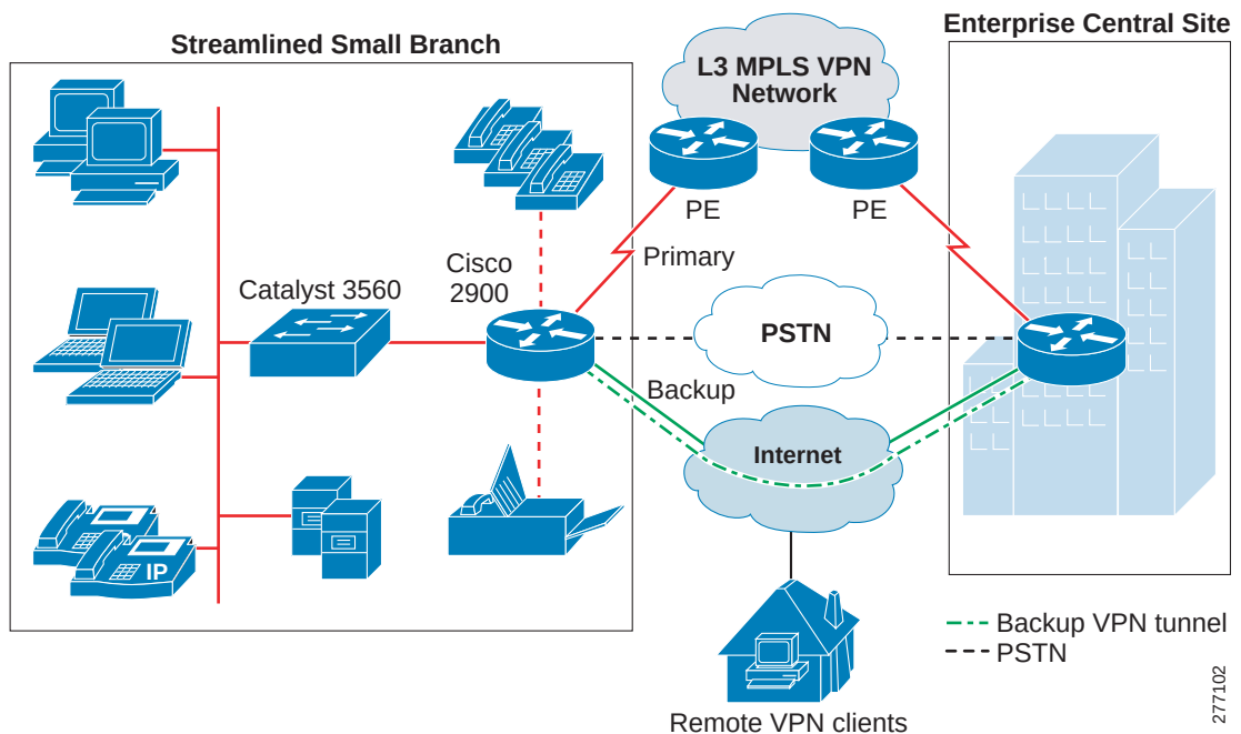
Figure 17 Streamlined Small Branch Network L3VPN Deployment
