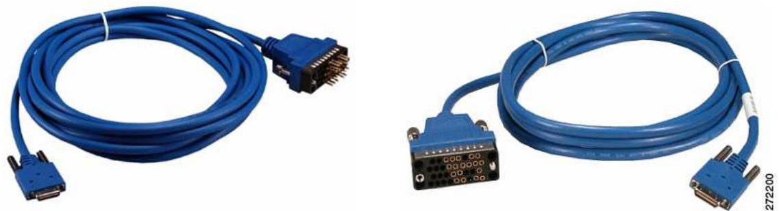
Figure 14 Male (CAB-SS-V35MC) and Female (CAB-SS-V35FC) V.35 Connectors
