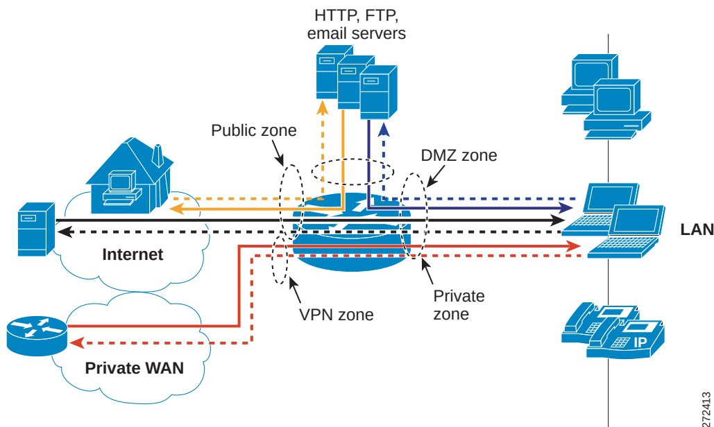
Figure 37 Security Zones
