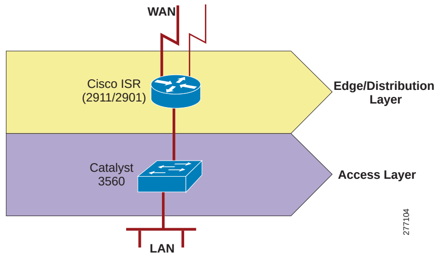
Figure 20 Hierarchical LAN Design
