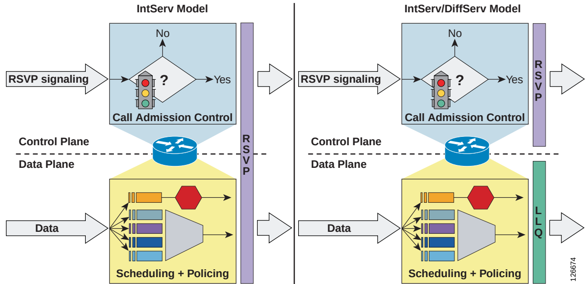
Figure 52 RSVP Operational Models: IntServ and IntServ/DiffServ
