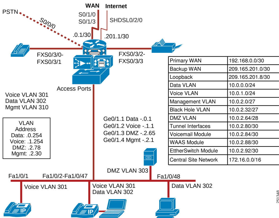
Figure 2 Services Ready Small Branch Network Topology
