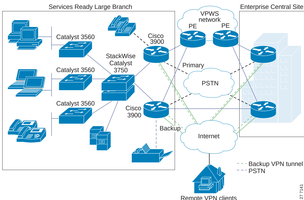
Figure 21 The Services Ready Large Branch Network VPWS Deployment
