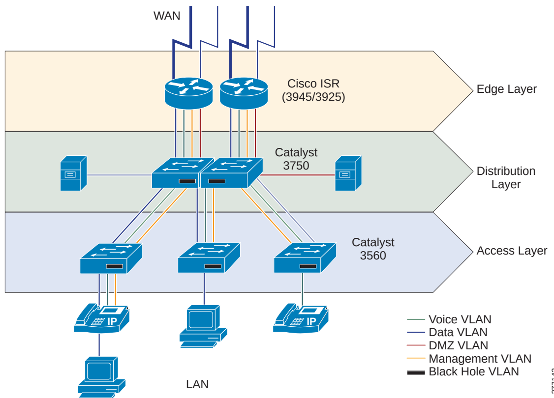
Figure 24 VLAN Design
