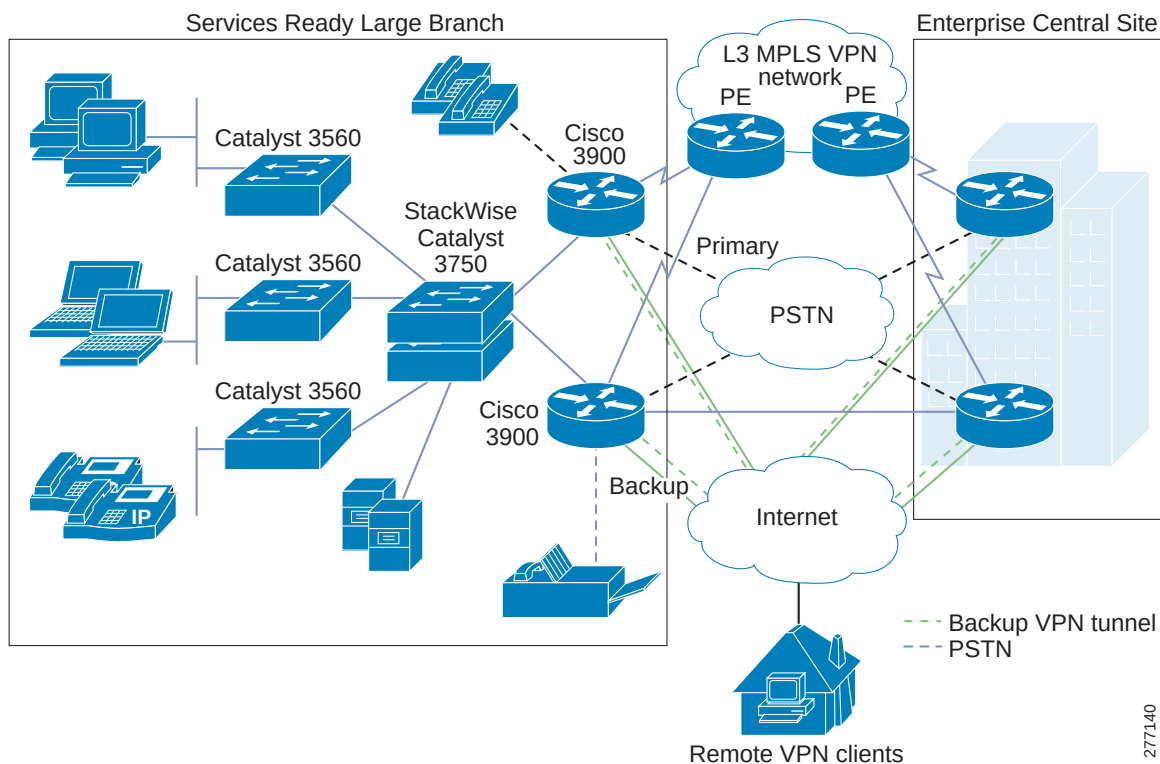
Figure 20 Services Ready Large Branch Network L3VPN Deployment
