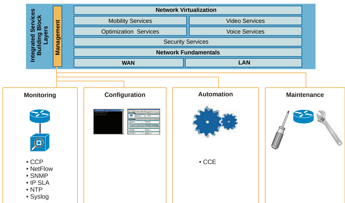
Figure 43 Management Services for a Branch Network
