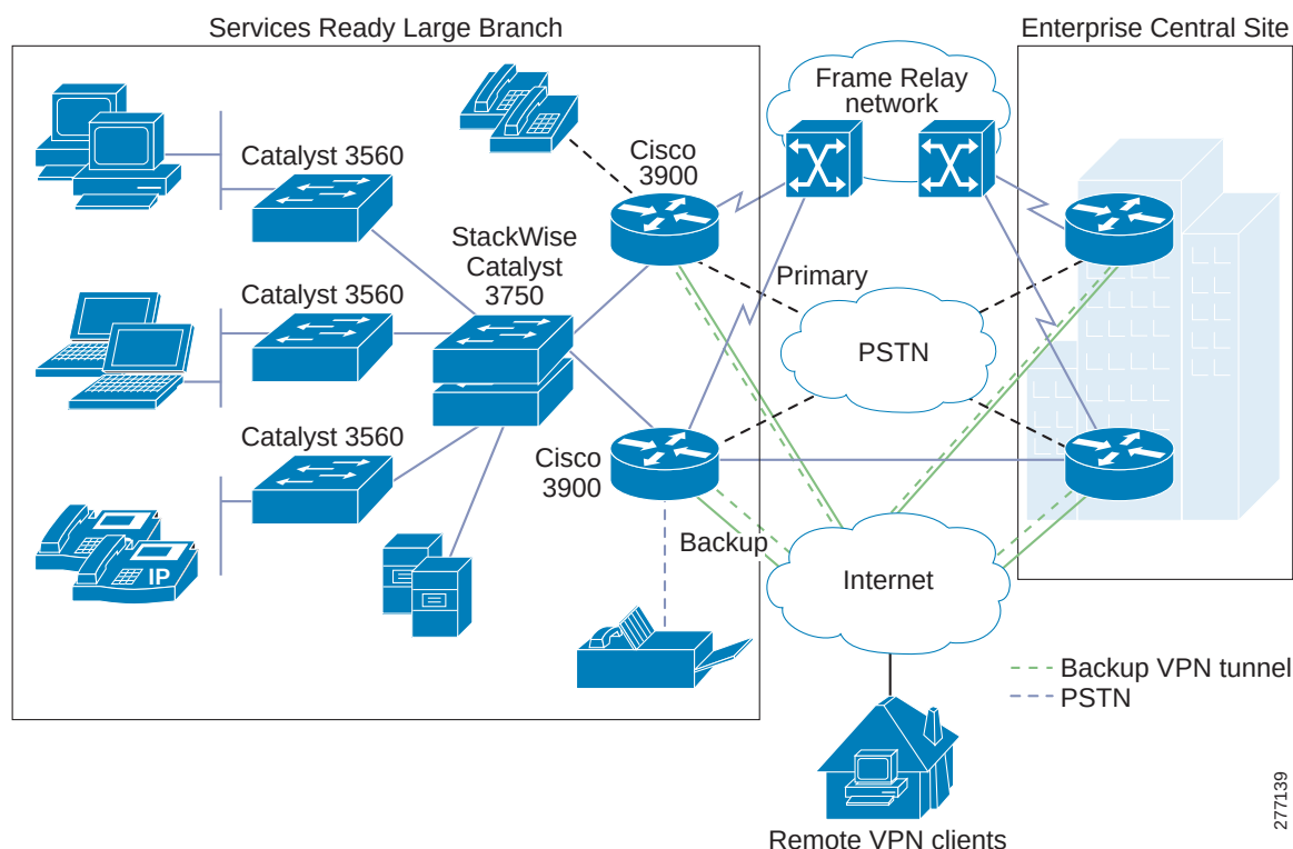
Figure 19 Services Ready Large Branch Network Frame Relay Service Deployment
