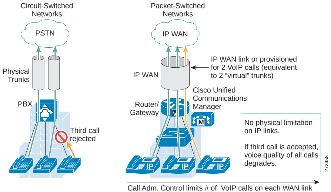
Figure 56 Traditional Versus VoIP Call Admission Control
