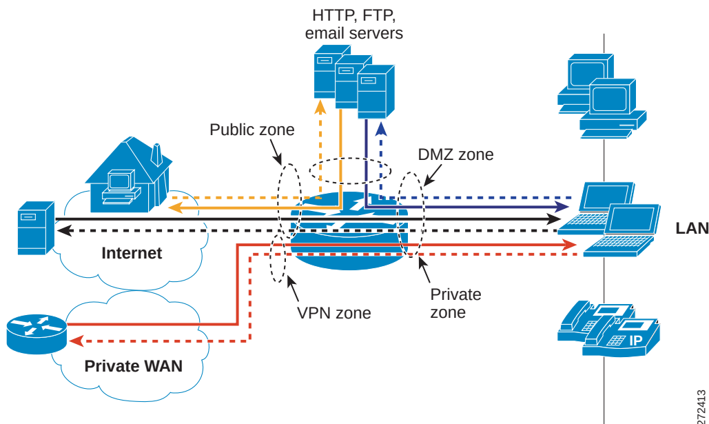
Figure 42 Security Zones
