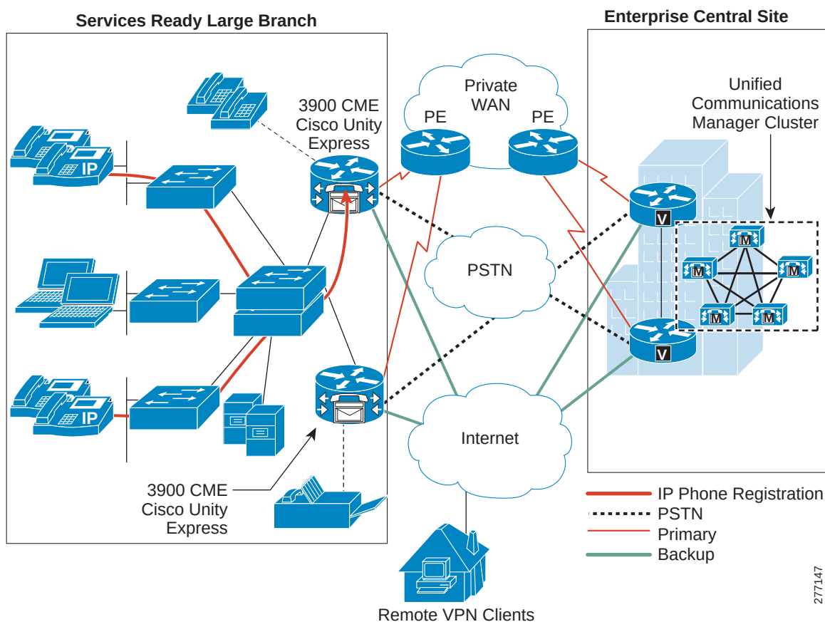
Figure 52 Distributed Call Control Model
