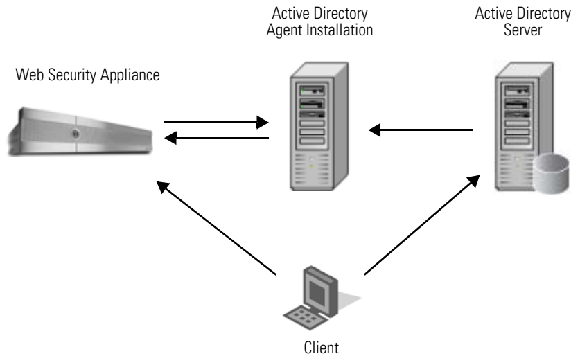
Figure 8-4 Active Directory Agent Workflow
