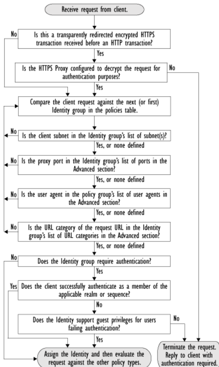
Figure 8-2 Policy Group Flow Diagram for Identities - Cookie-Based Surrogates
