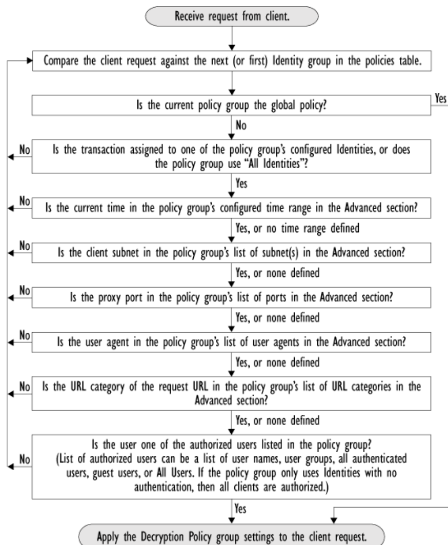
Figure 11-3 Policy Group Flow Diagram for Decryption Policies
