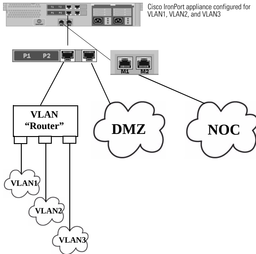
Figure 25-2 Using VLANs to Increase the Number of Networks Available on the Appliance
