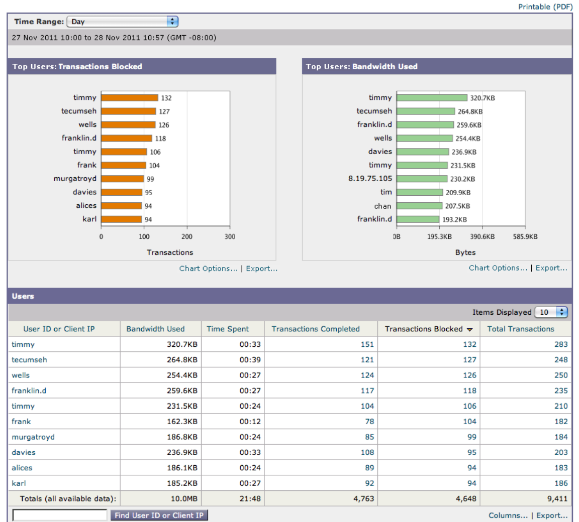
Figure 23-2 The Users Page
