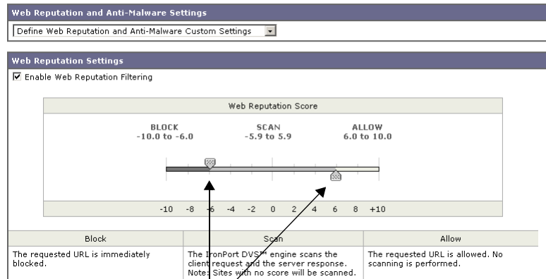
Figure 19-1 Web Reputation Filter Settings for Access Policies
