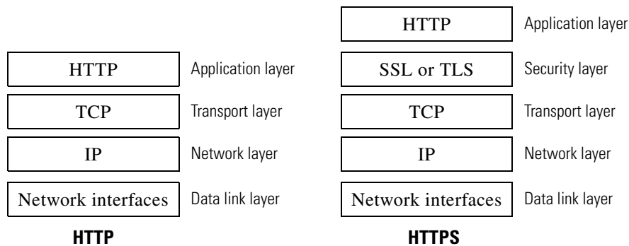
Figure A-1 HTTPS and HTTP OSI Layers
