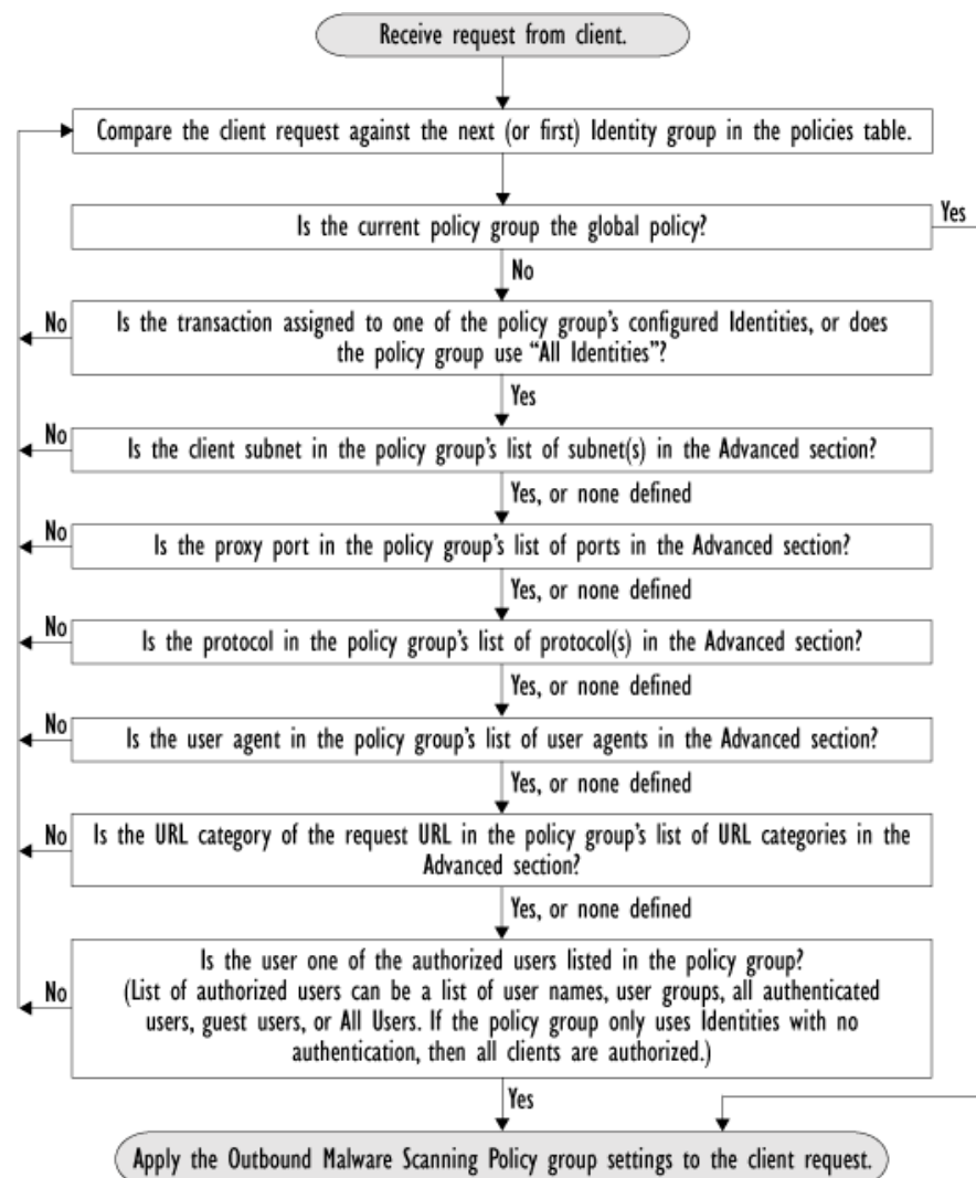
Figure 13-1 Policy Group Flow Diagram for Outbound Malware Scanning Policies
