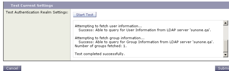
Figure 21-5 Authentication Testing Results
