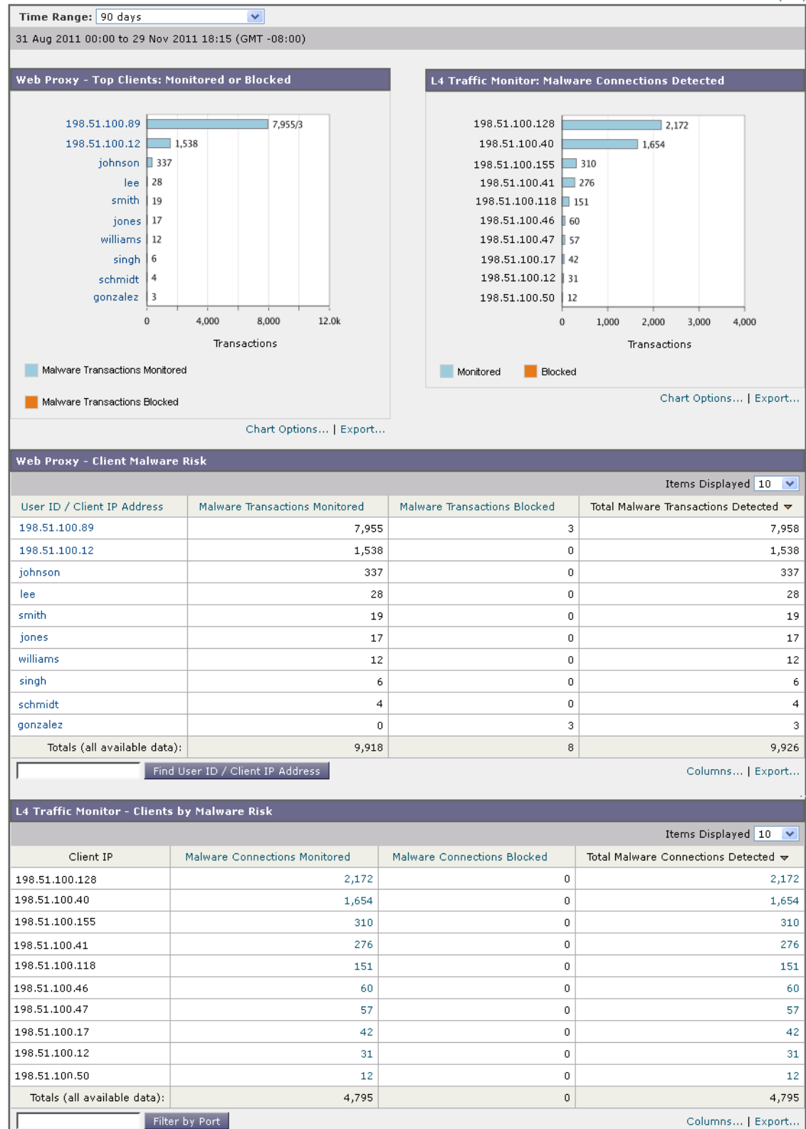
Figure 24-10 Client Malware Risk Page Client Malware Risk
