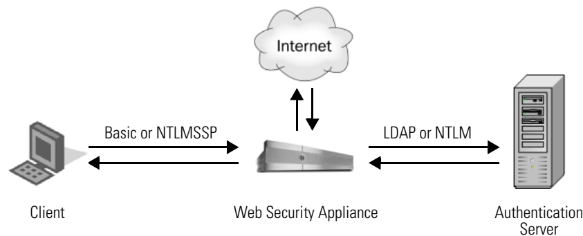
Figure 21-1 Web Security Appliance Authentication
