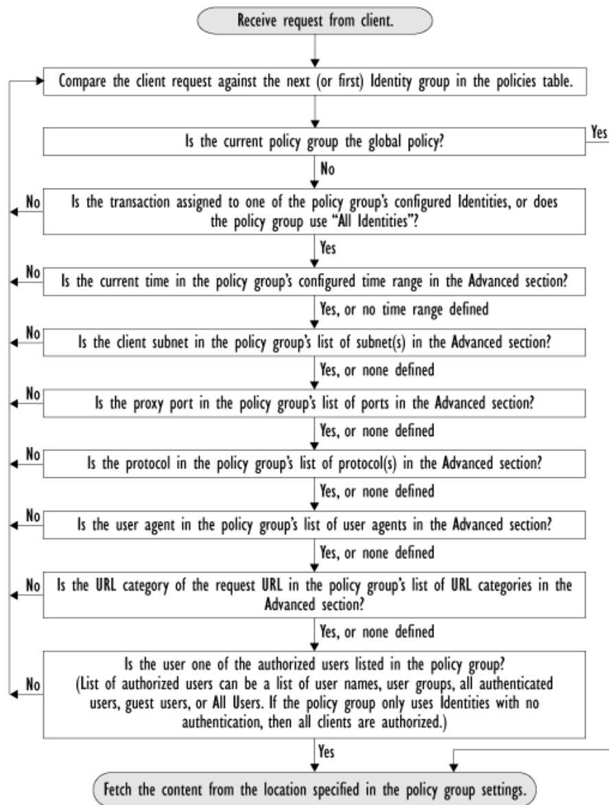
Figure 11-2 Policy Group Flow Diagram for Routing Policies
