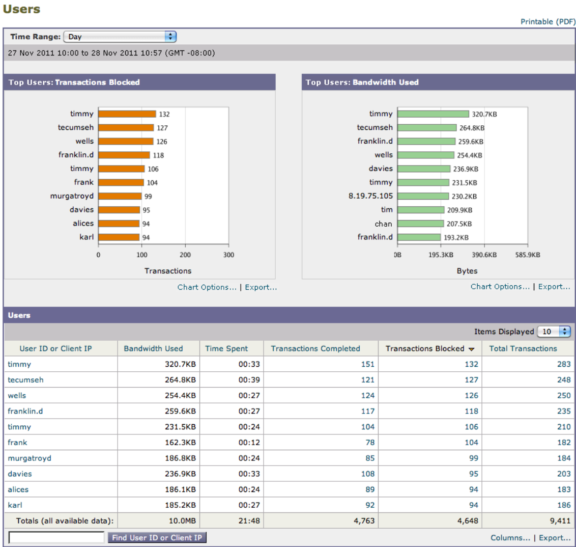
Figure 24-2 The Users Page
