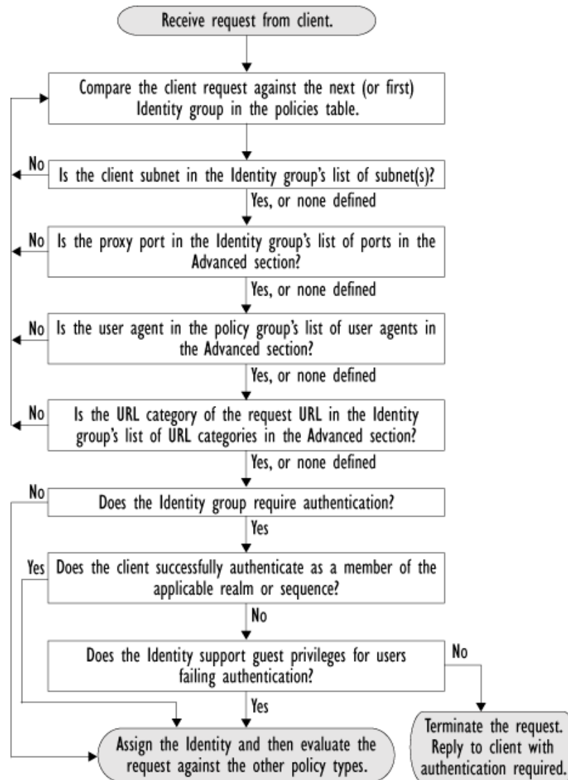
Figure 9-2 Policy Group Flow Diagram for Identities - No Surrogates and IP-Based Surrogates
