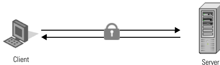
Figure 12-3 HTTPS Connection
