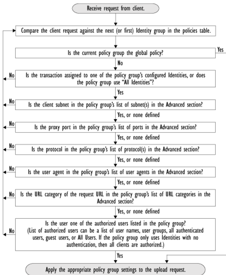
Figure 14-1 Policy Group Flow Diagram for Data Security and External DLP Policies
