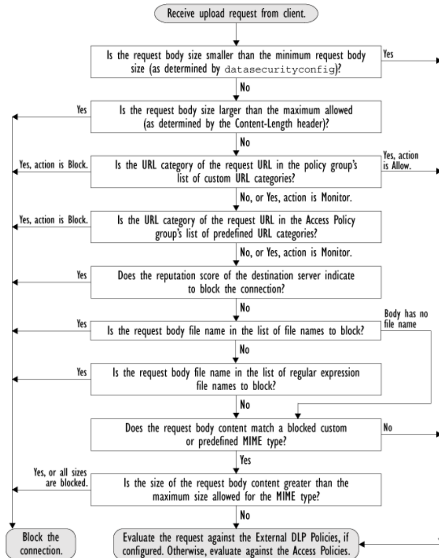
Figure 14-3 Applying Data Security Policy Actions
