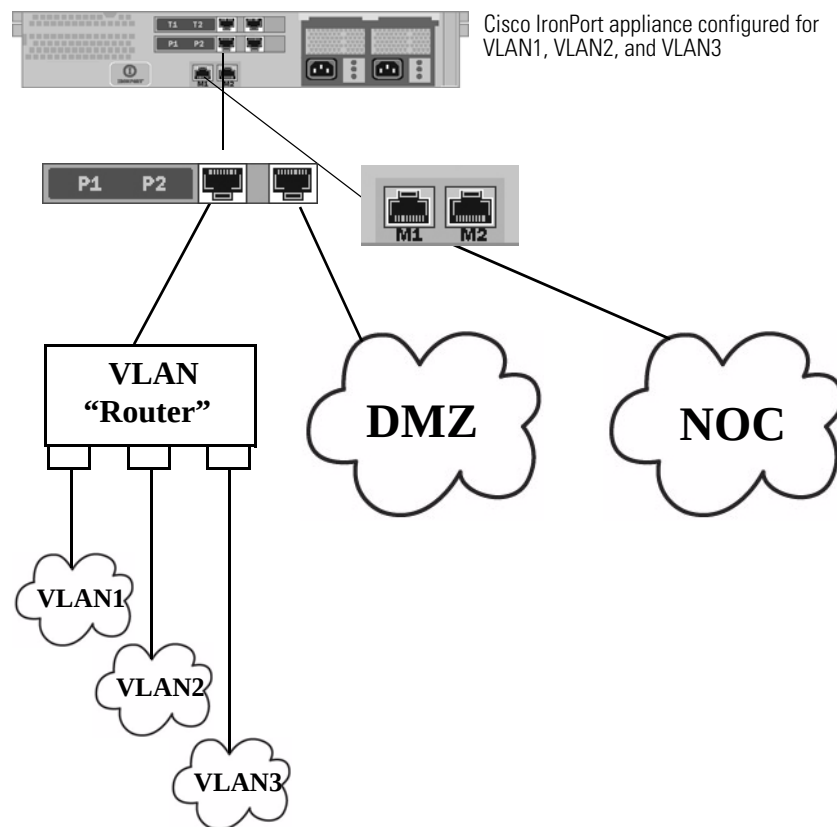
Figure 26-4 Using VLANs to Increase the Number of Networks Available on the Appliance
