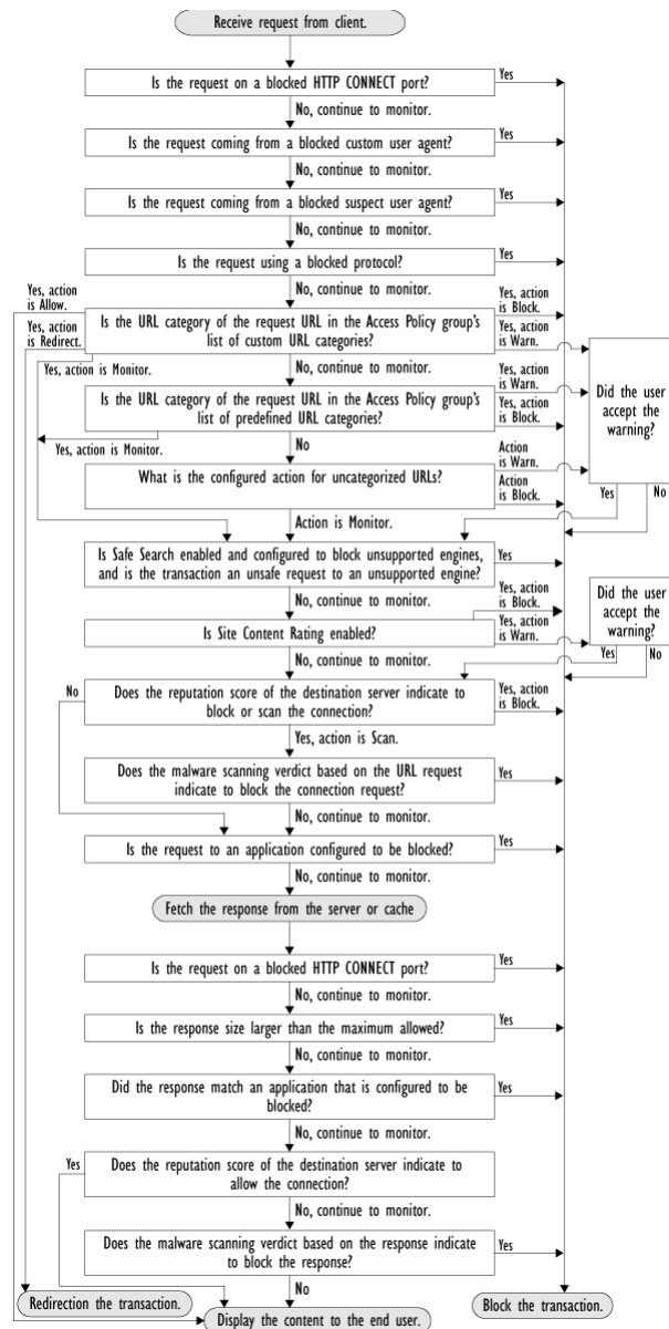
Figure 10-3 Applying Access Policy Actions
