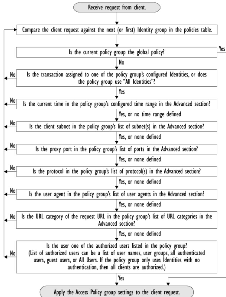
Figure 10-1 Policy Group Flow Diagram for Access Policies
