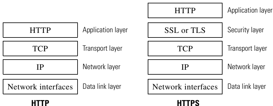
Figure 12-1 HTTPS and HTTP OSI Layers
