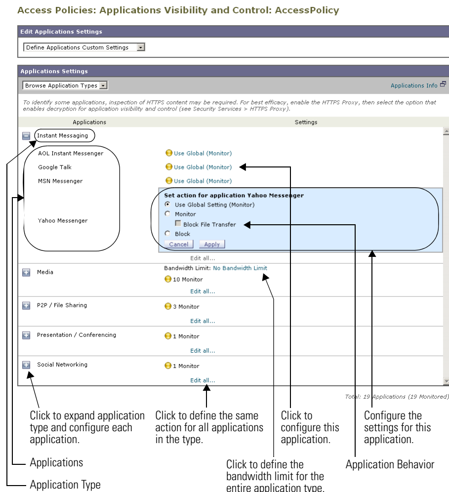
Figure 19-1 Configuring Applications for a User Defined Access Policy—Browse View
