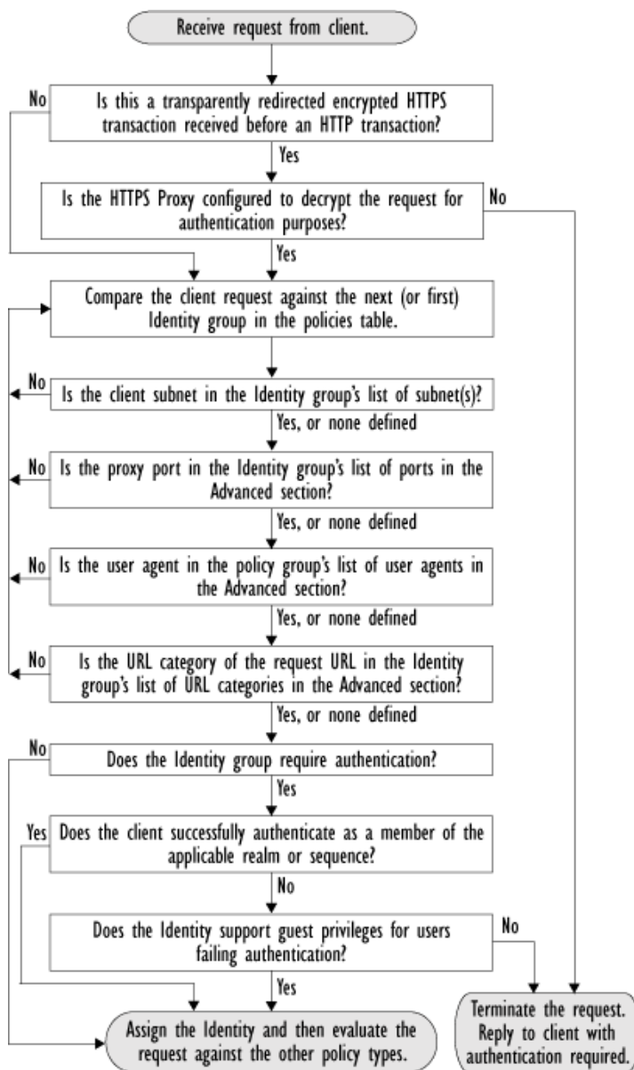
Figure 7-3 Policy Group Flow Diagram for Identities - Cookie-Based Surrogates
