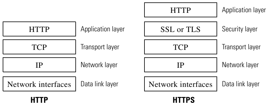
Figure 10-1 HTTPS and HTTP OSI Layers
