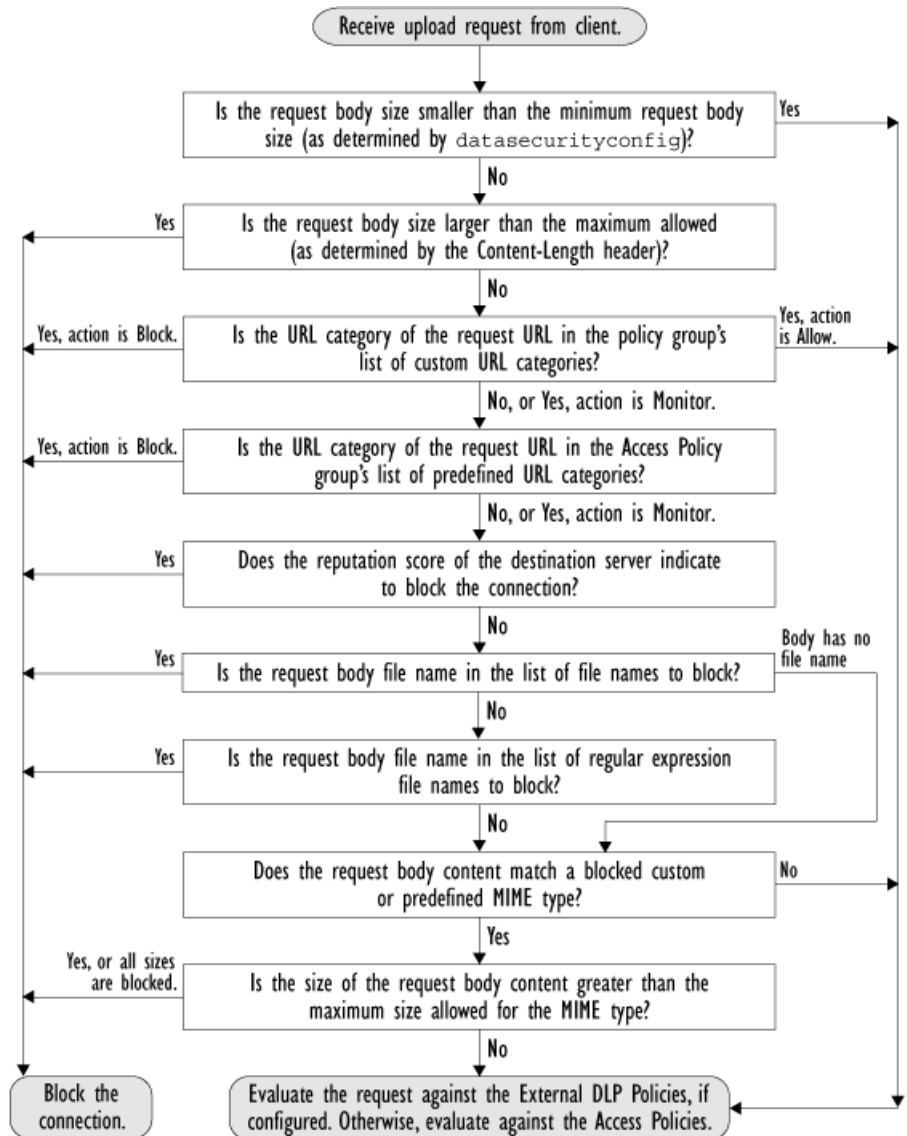
Figure 12-3 Applying Data Security Policy Actions
