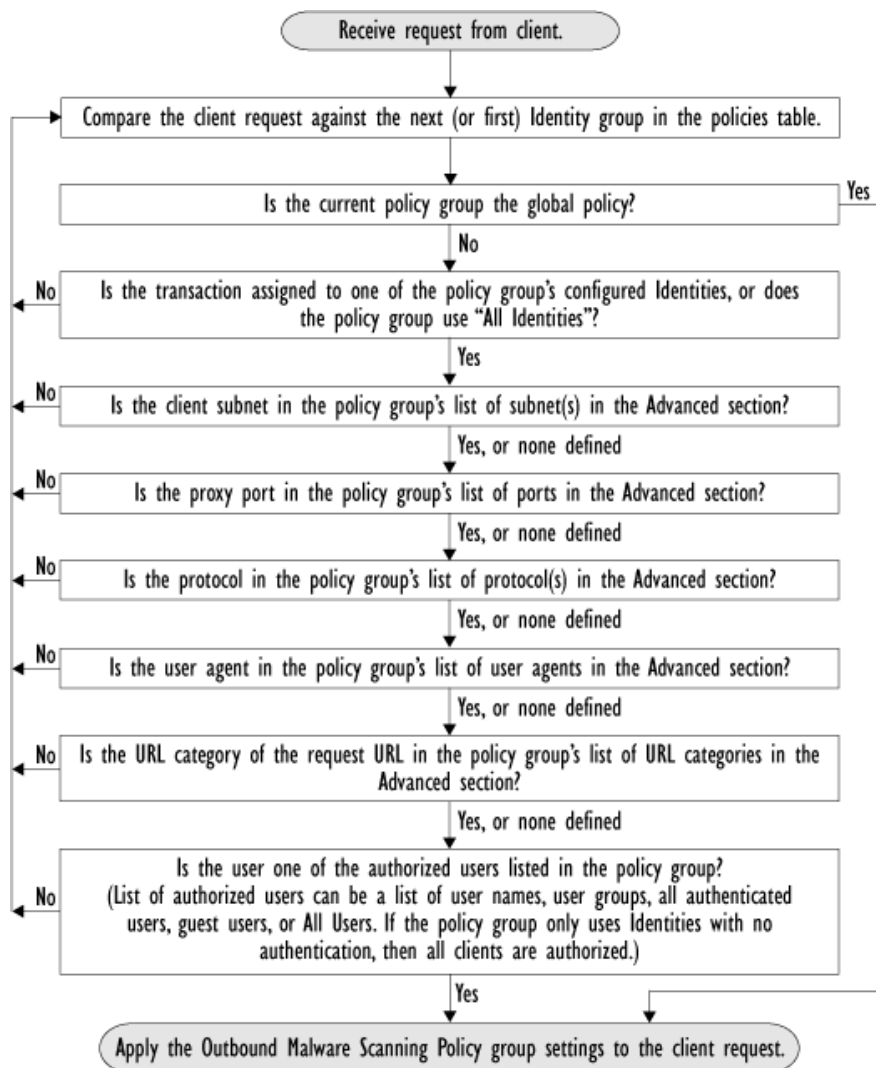
Figure 11-1 Policy Group Flow Diagram for Outbound Malware Scanning Policies
