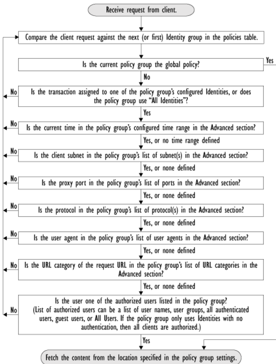
Figure 9-2 Policy Group Flow Diagram for Routing Policies
