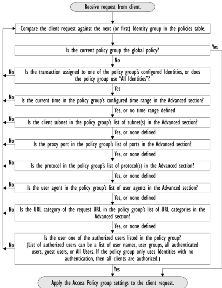
Figure 8-1 Policy Group Flow Diagram for Access Policies
