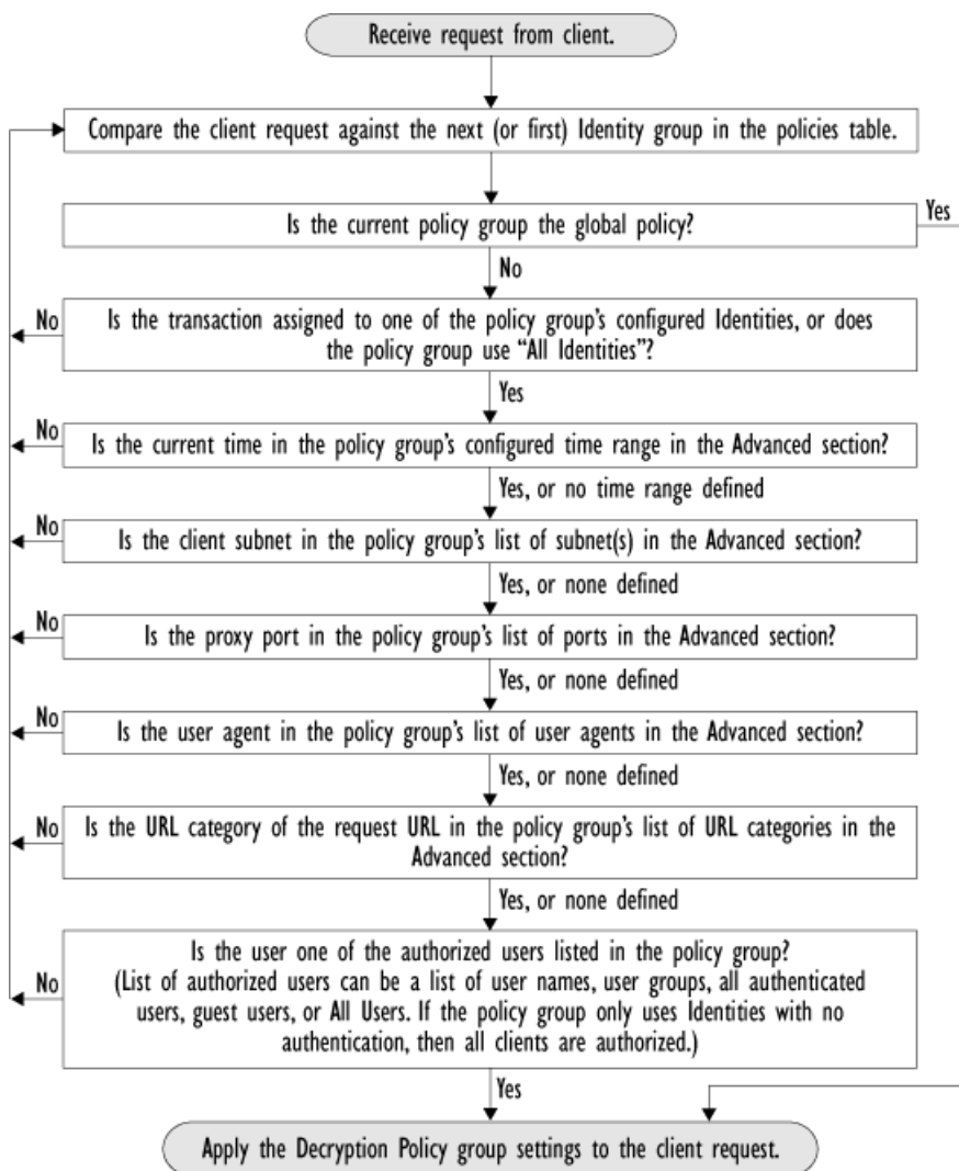
Figure 10-7 Policy Group Flow Diagram for Decryption Policies
