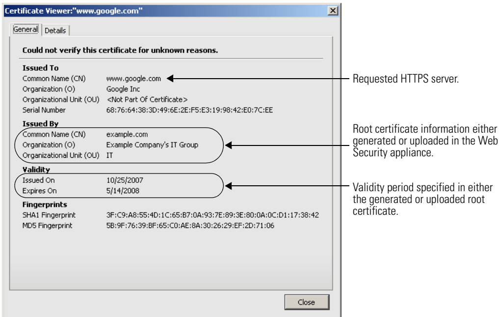
Figure 10-6 Certificate Issued by Web Security Appliance
