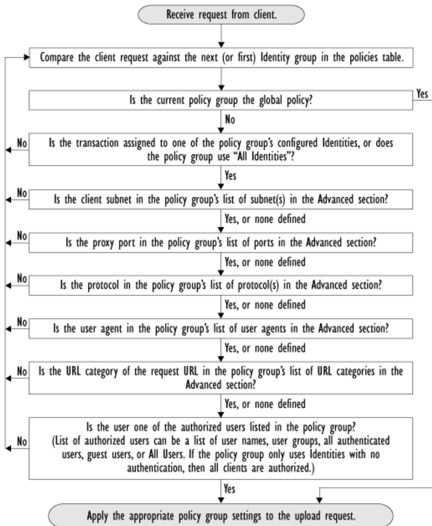
Figure 12-1 Policy Group Flow Diagram for Data Security and External DLP Policies
