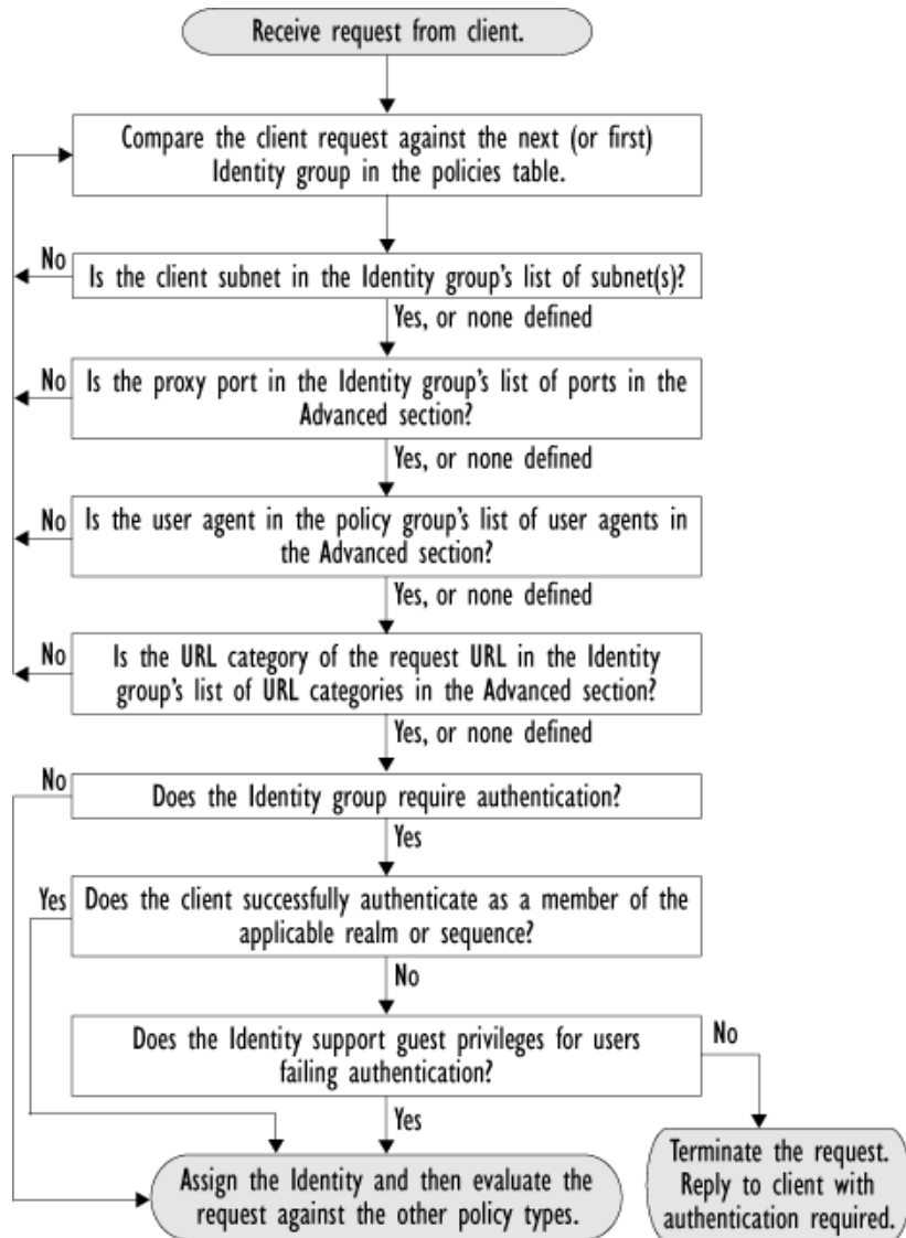
Figure 7-2 Policy Group Flow Diagram for Identities - No Surrogates and IP-Based Surrogates
