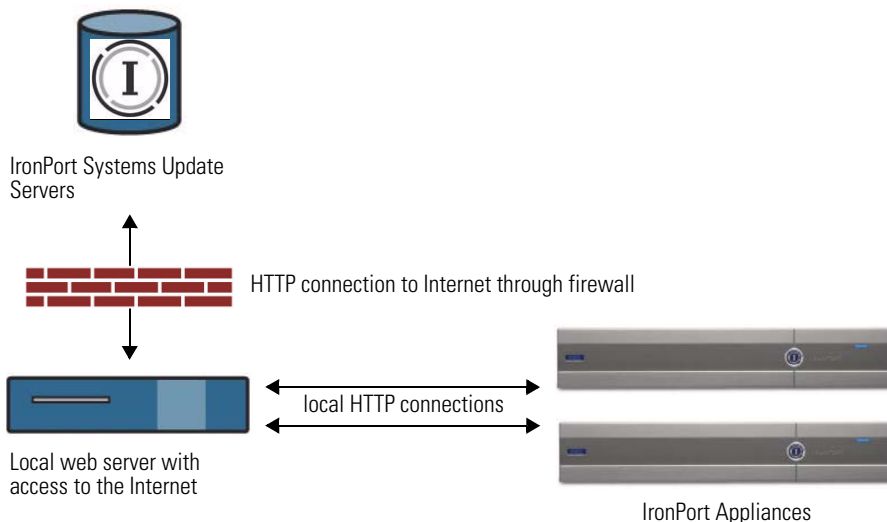
Figure 26-21 Upgrading from a Local Server
