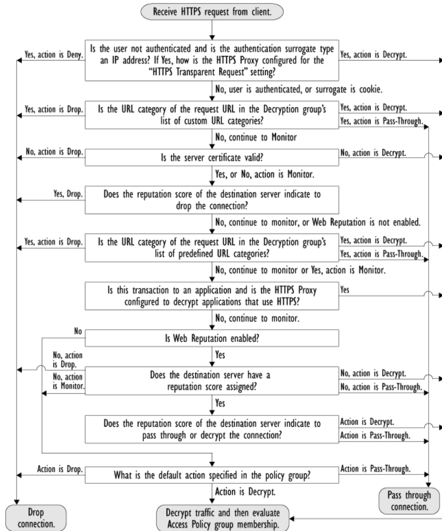
Figure 10-9 Applying Decryption Policy Actions
