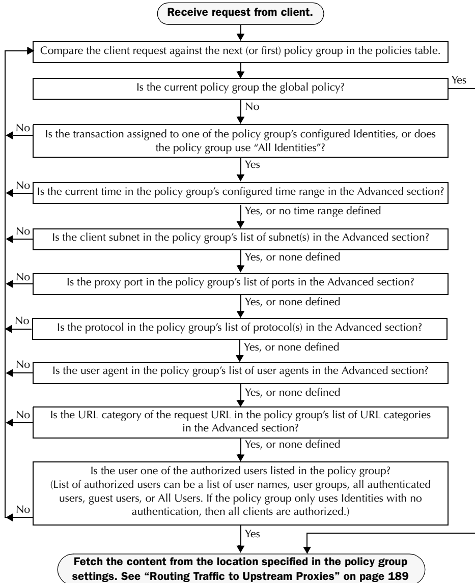
Figure 10-2 Policy Group Flow Diagram for Routing Policies
