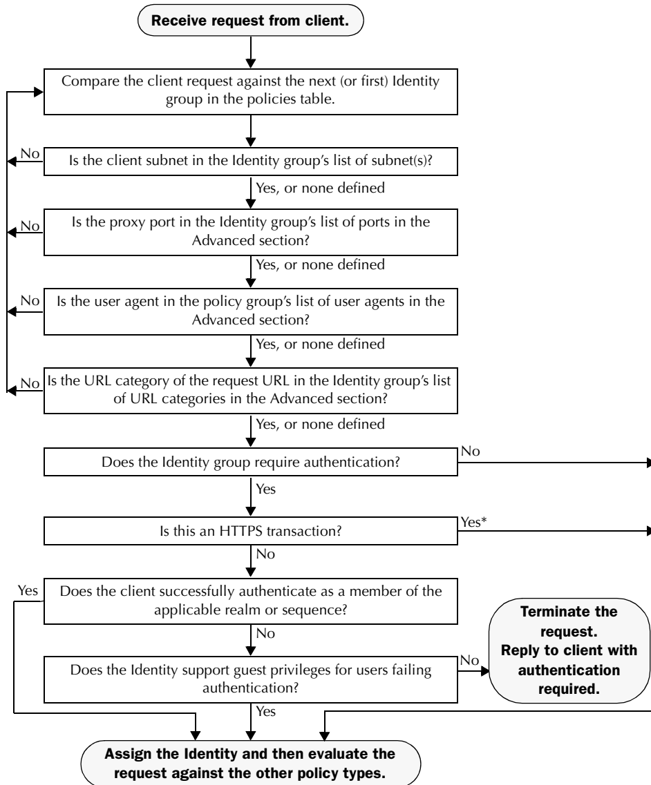
Figure 8-3 Policy Group Flow Diagram for Identities - Cookie-Based Surrogates
