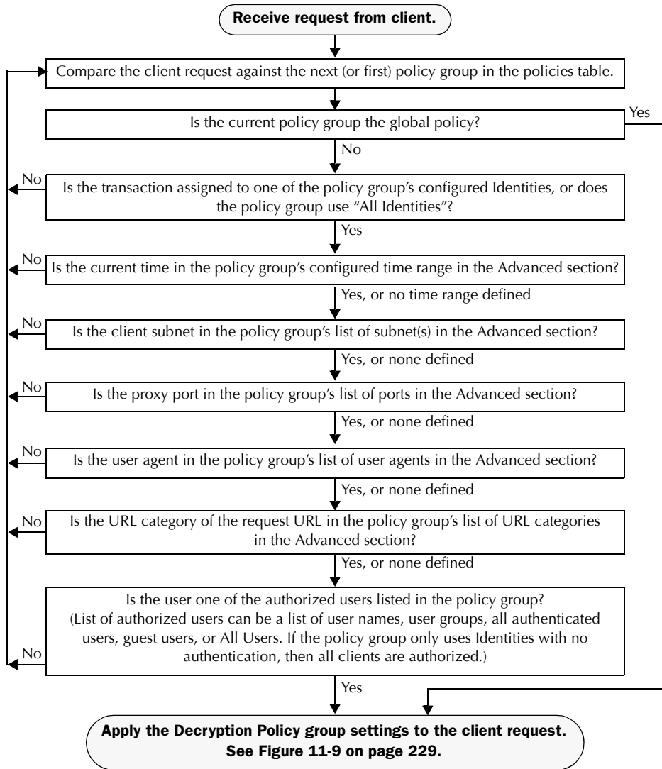
Figure 11-7 Policy Group Flow Diagram for Decryption Policies
