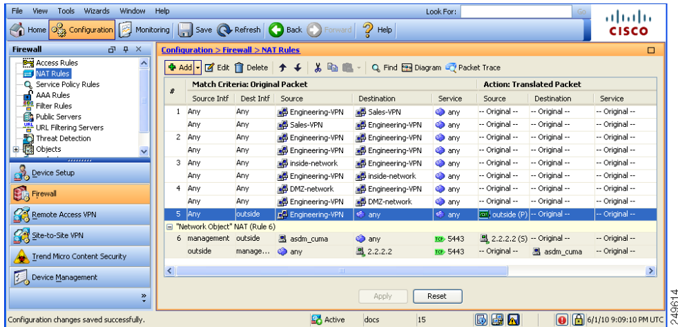
Figure 87-5 Unified NAT table
