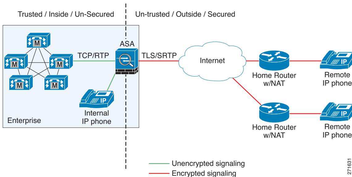
Figure 54-1 Phone Proxy Secure Deployment
