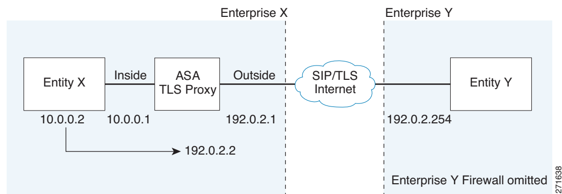
Figure 68-2 Abstracted Presence Federation Proxy Scenario between Two Server Entities
