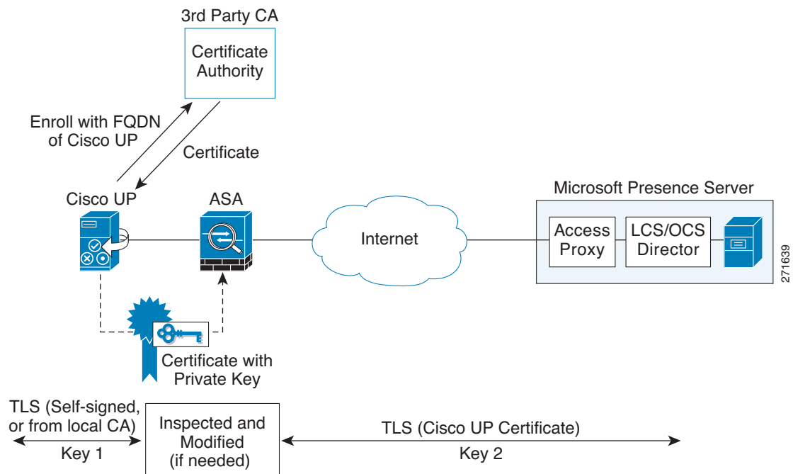
Figure 68-3 How the Security Appliance Represents Cisco Unified Presence – Certificate Impersonate
