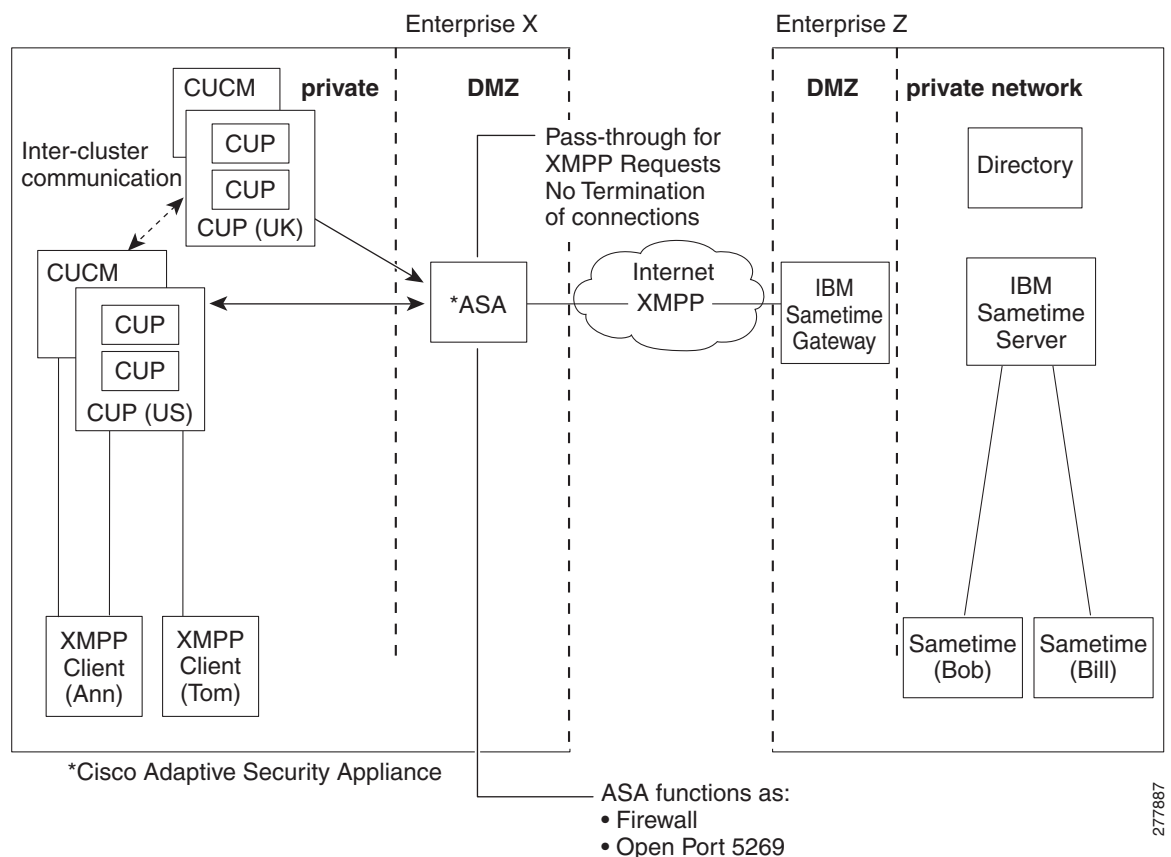
Figure 68-4 Basic XMPP Federated Network between Cisco Unified Presence and IBM Sametime
