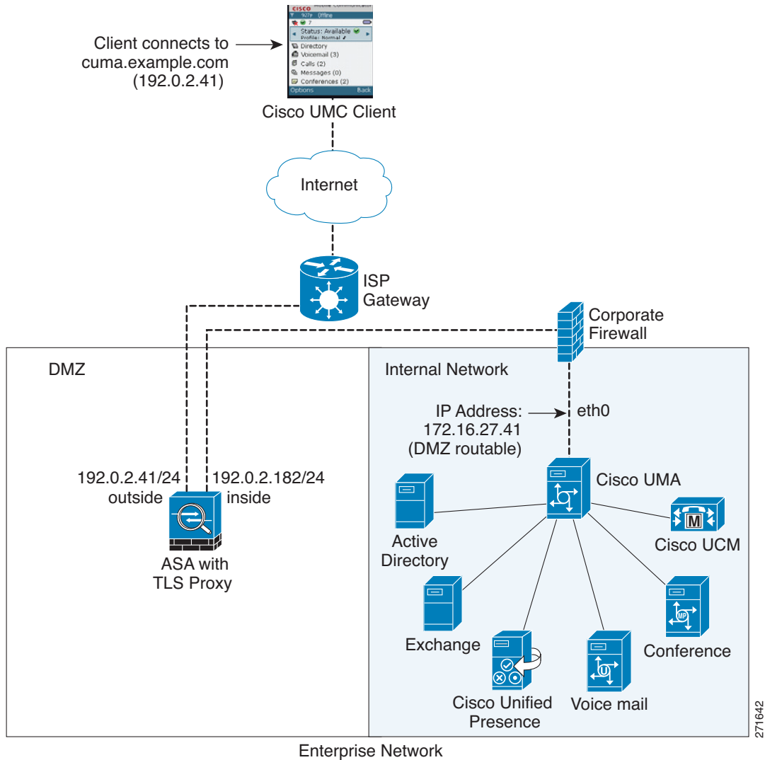
Figure 67-3 Cisco UMC/Cisco UMA Architecture – Scenario 2: Security Appliance as Mobility Advantage Proxy Only
