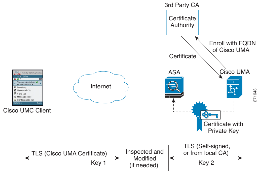
Figure 67-4 How the Security Appliance Represents Cisco UMA – Private Key Sharing
