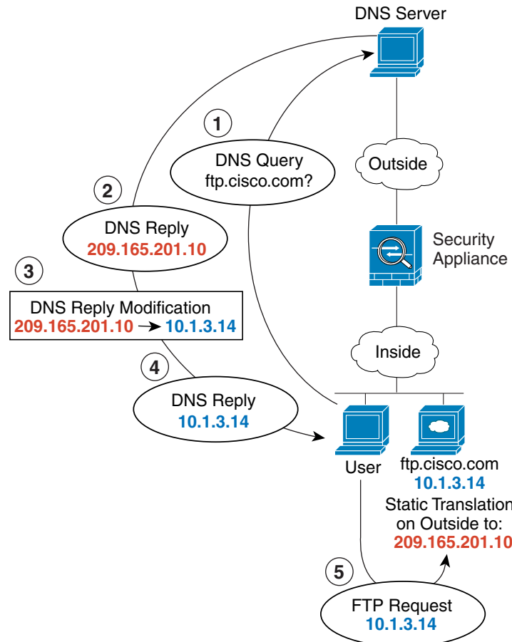
Figure 32-26 DNS Reply Modification, DNS Server on Outside
