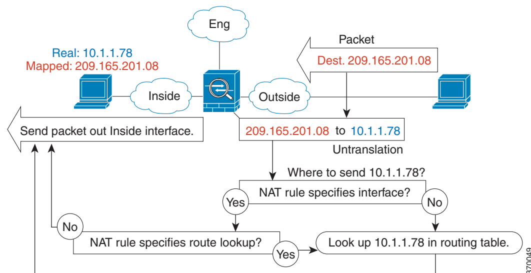
Figure 32-20 Routed Mode Egress Interface Selection
