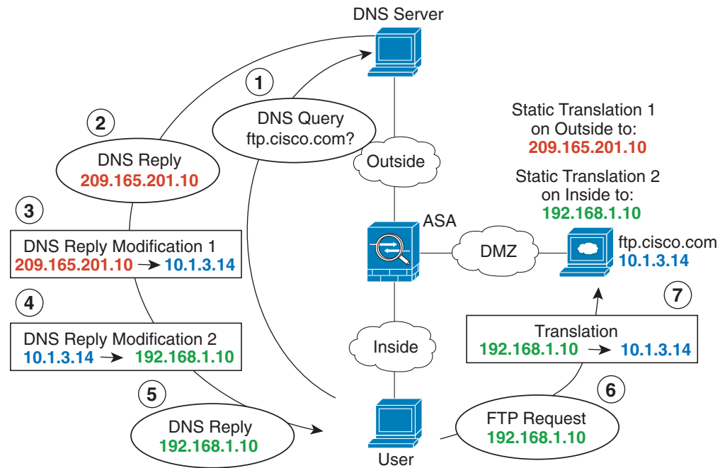
Figure 32-27 DNS Reply Modification, DNS Server, Host, and Server on Separate Networks
