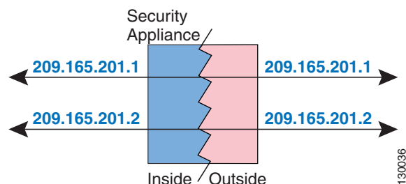
Figure 32-11 Identity NAT
