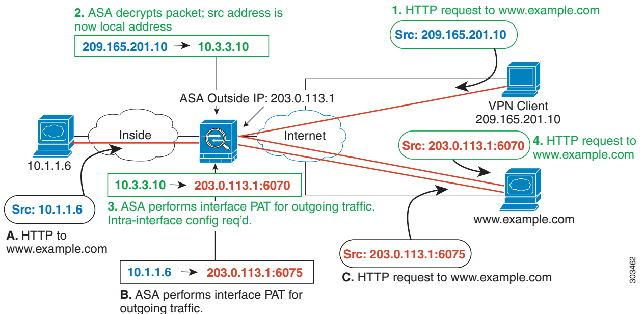
Figure 32-21 Interface PAT for Internet-Bound VPN Traffic (Intra-Interface)
