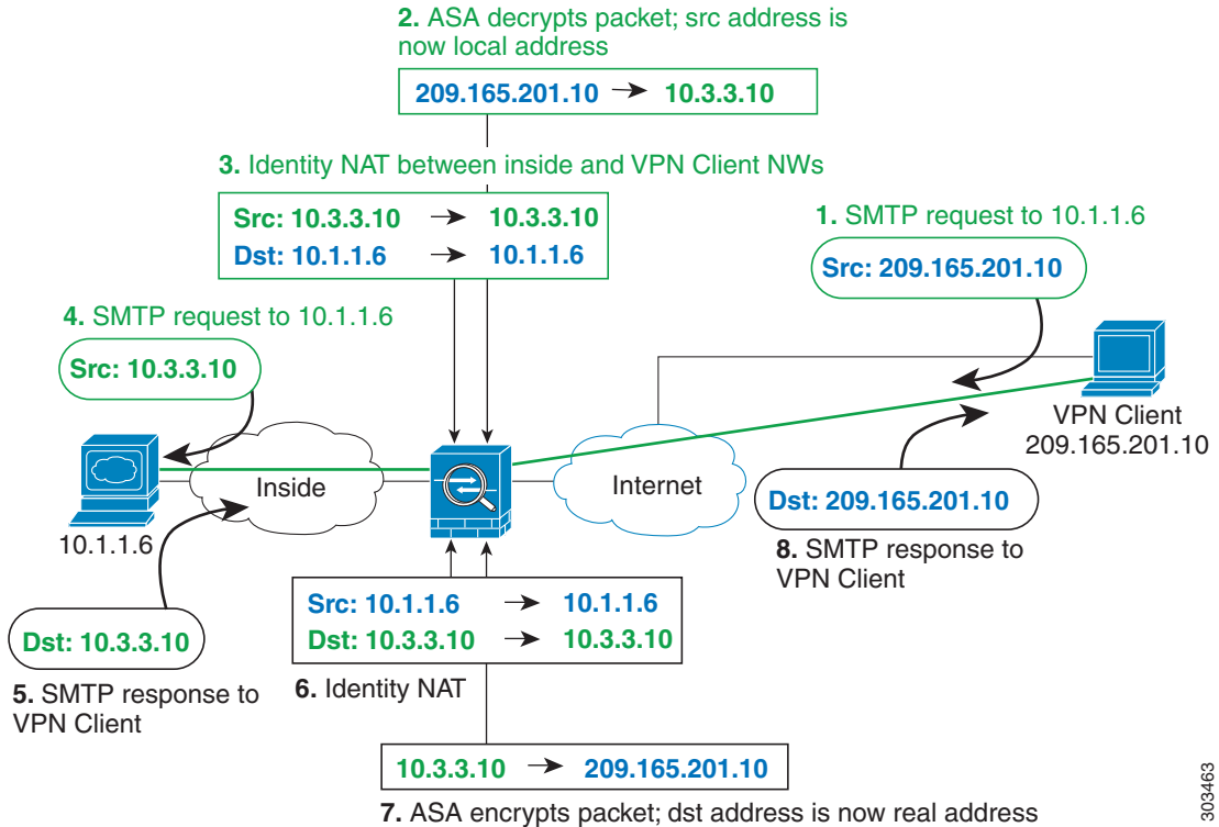
Figure 32-22 Identity NAT for VPN Clients
