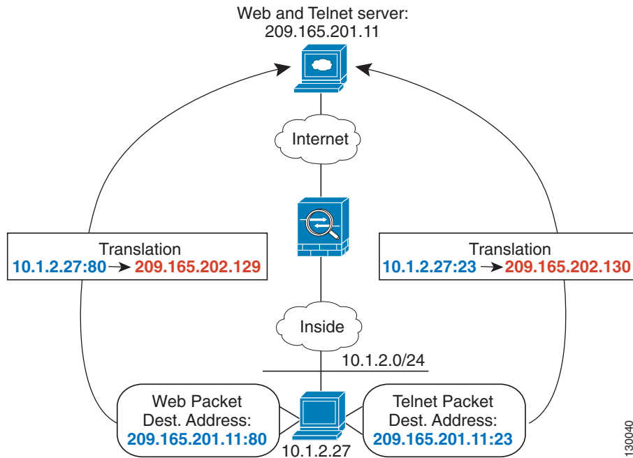
Figure 32-15 Twice NAT with Different Destination Ports
