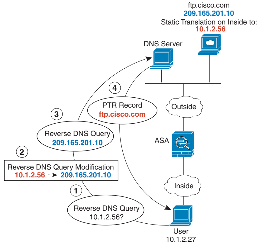
Figure 32-30 PTR Modification, DNS Server on Host Network
