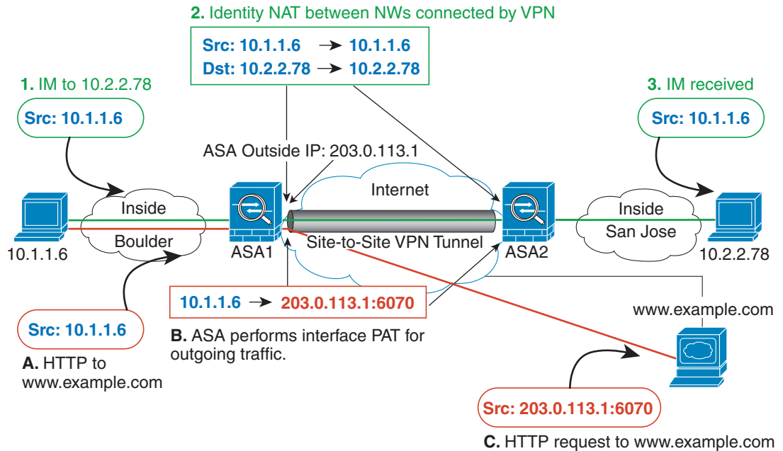
Figure 32-23 Interface PAT and Identity NAT for Site-to-Site VPN
