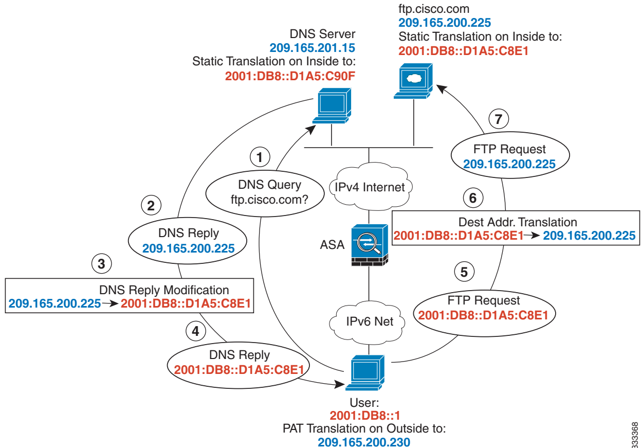
Figure 32-29 DNS64 Reply Modification Using Outside NAT
