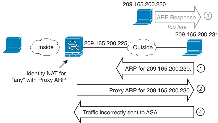
Figure 32-18 Proxy ARP Problems with Identity NAT
