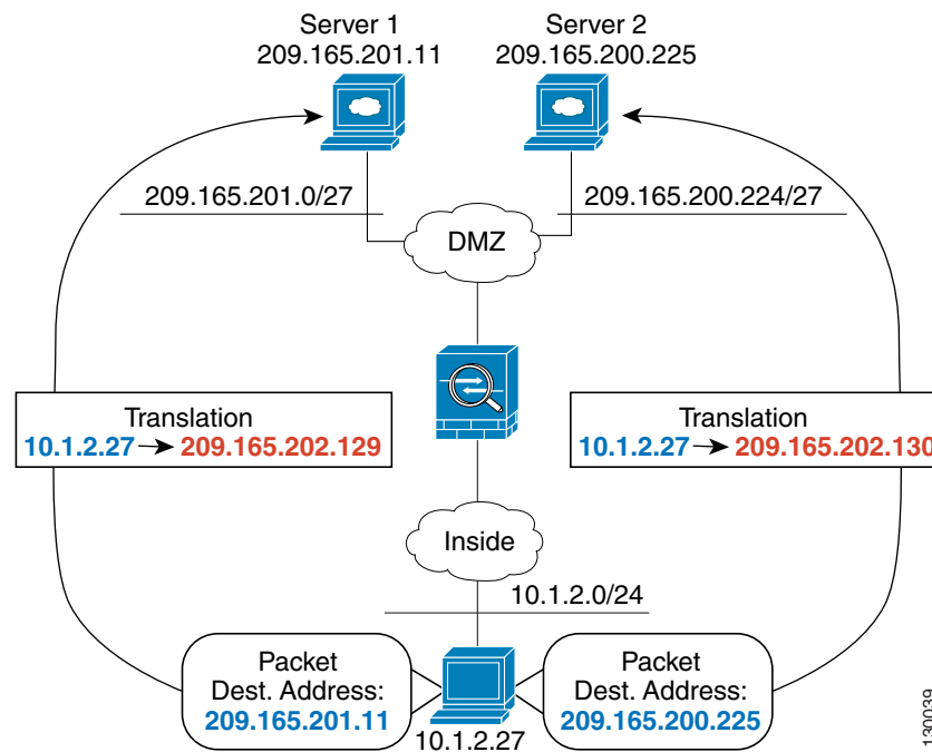
Figure 32-14 Twice NAT with Different Destination Addresses
