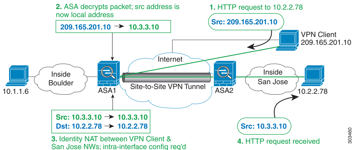
Figure 32-24 VPN Client Access to Site-to-Site VPN
