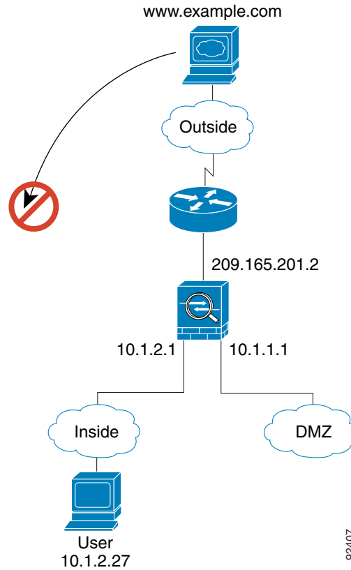
Figure 4-6 Outside to Inside
