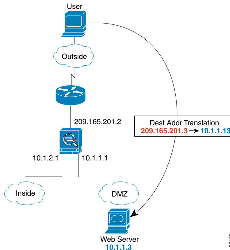
Figure 4-4 Outside to DMZ
