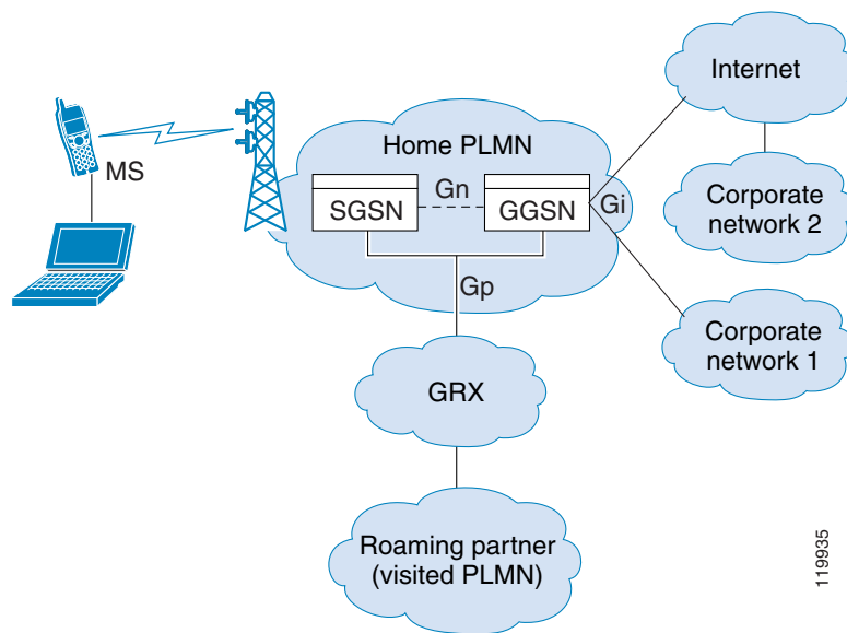
Figure 61-1 GPRS Tunneling Protocol
