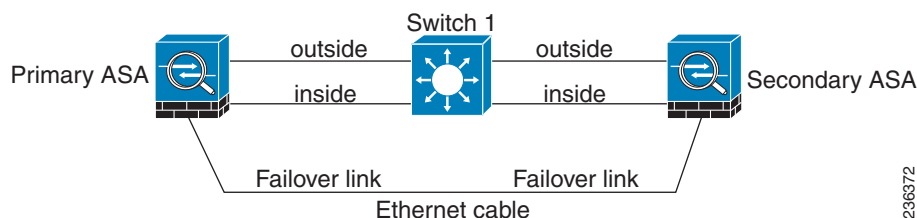
Figure 11-4 Connecting with a Cable
