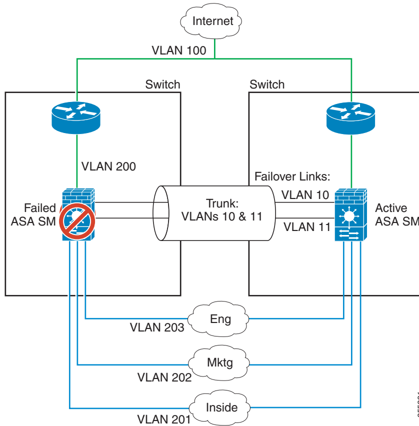
Figure 11-10 ASASM Failure
