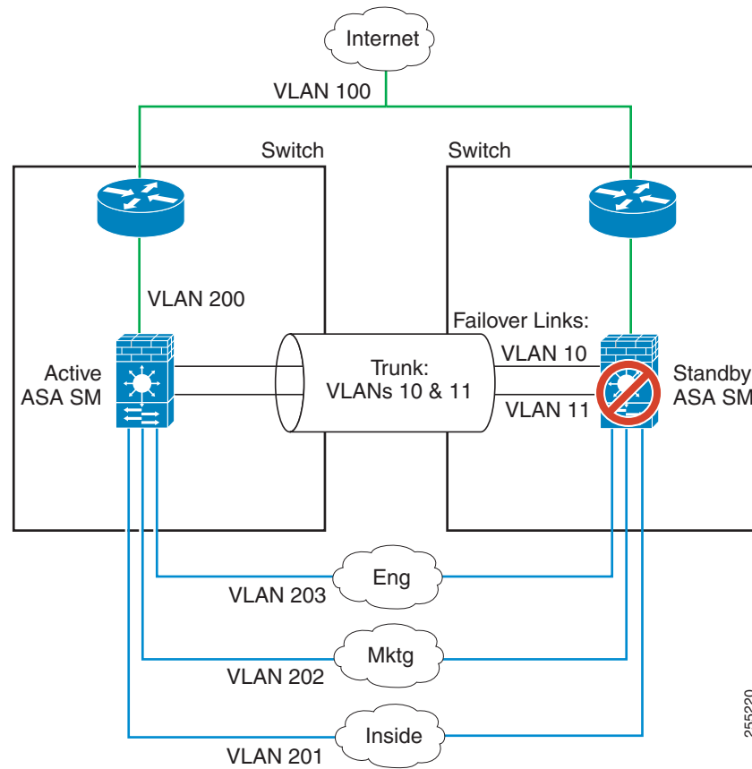
Figure 11-9 Normal Operation
