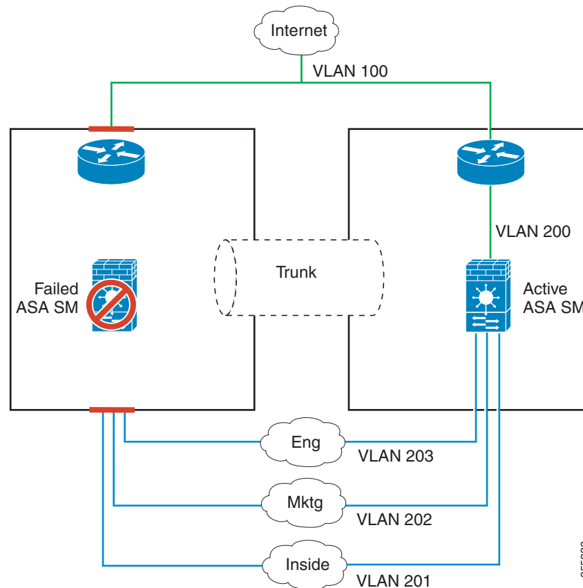
Figure 11-11 Switch Failure
