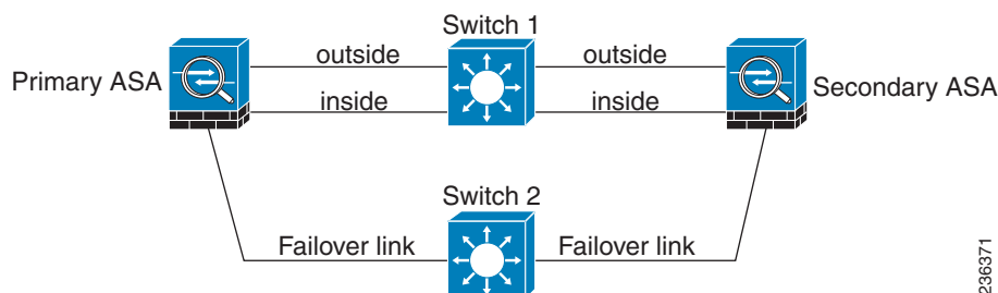
Figure 11-3 Connecting with a Different Switch
