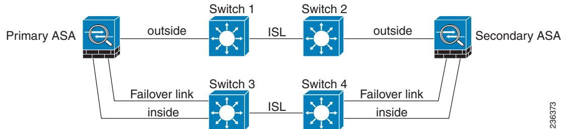
Figure 11-5 Connecting with a Secure Switch
