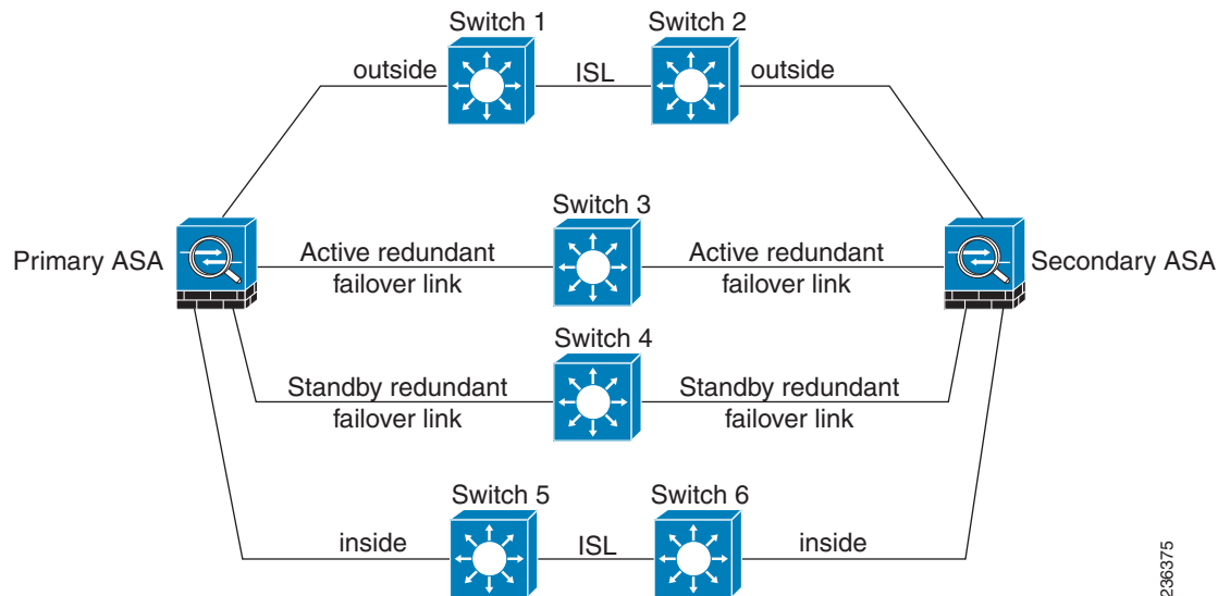
Figure 11-6 Connecting with Redundant Interfaces
