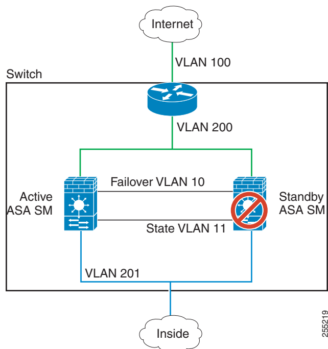
Figure 11-8 Intra-Switch Failover
