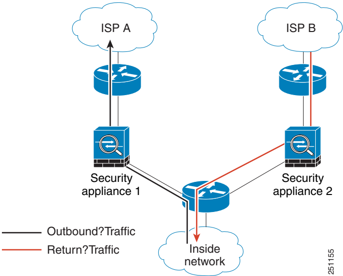
Figure 71-1 Asymmetric Routing
