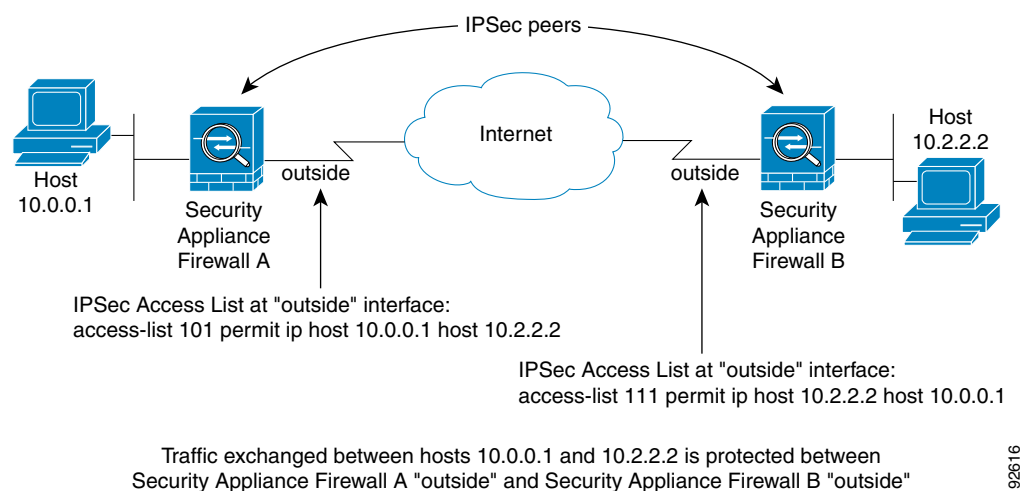
Figure 60-4 How Crypto Access Lists Apply to IPsec
