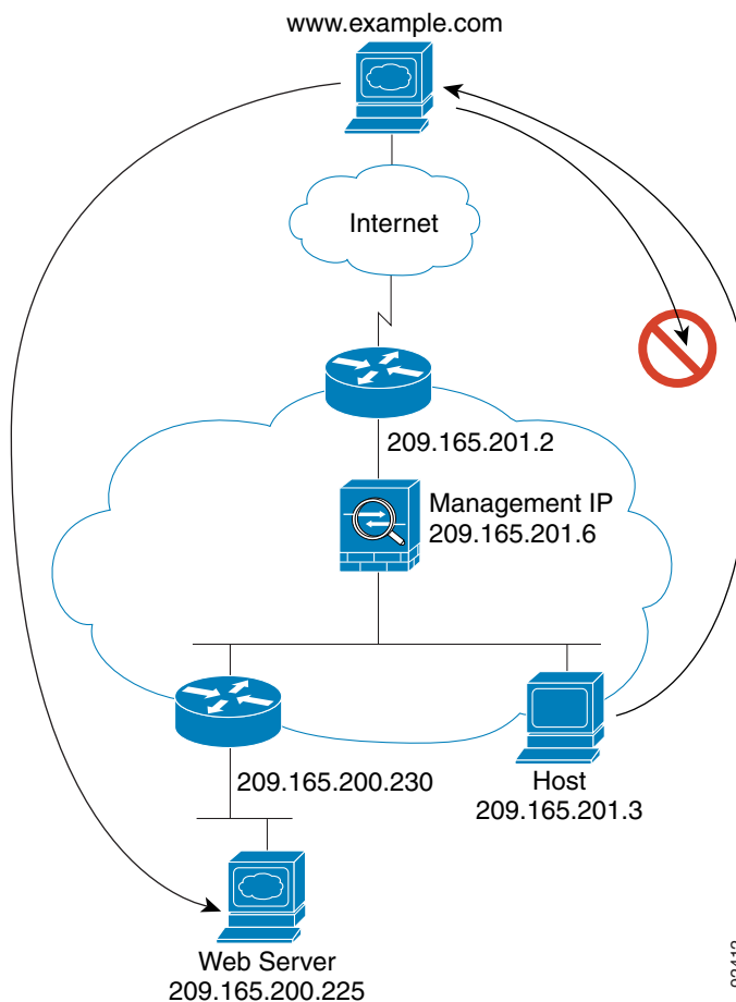
Figure 4-7 Typical Transparent Firewall Data Path
