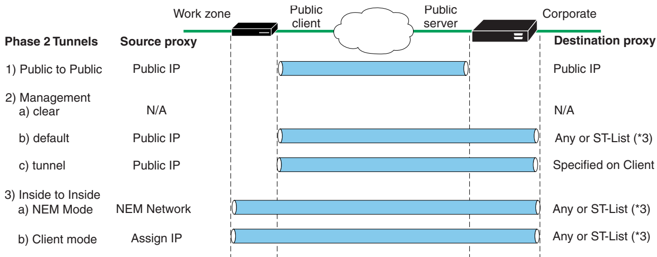
Figure 67-1 Easy VPN Hardware Client Tunneling Options for the Cisco ASA 5505
