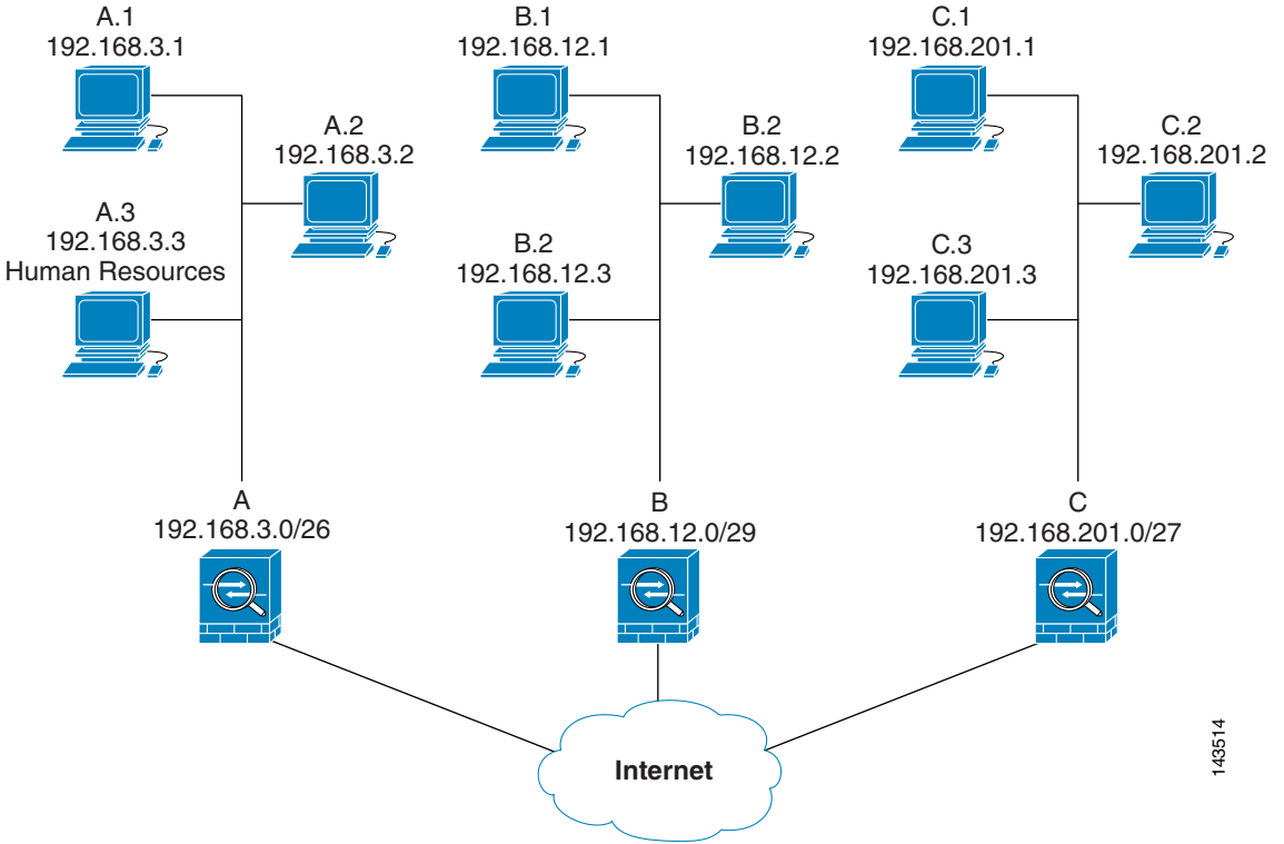
Figure 61-3 Effect of Permit and Deny ACEs on Traffic (Real Addresses)
