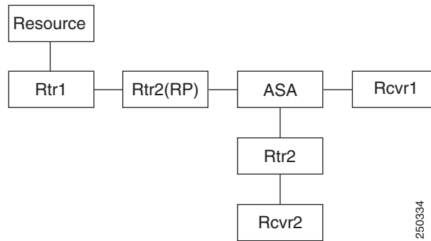
Figure A-8 Multicast Routing Configuration
