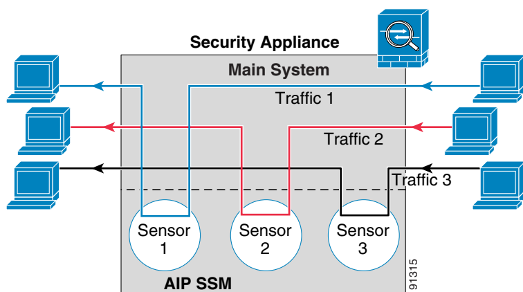
Figure 23-4 Single Mode Security Appliance with Multiple Virtual Sensors
