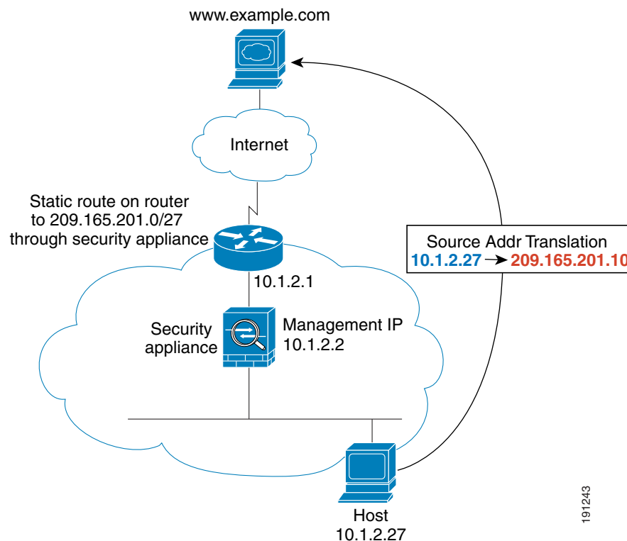
Figure 17-9 Inside to Outside with NAT
