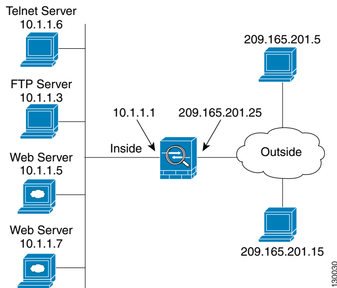
Figure 19-29 Port Redirection Using Static PAT
