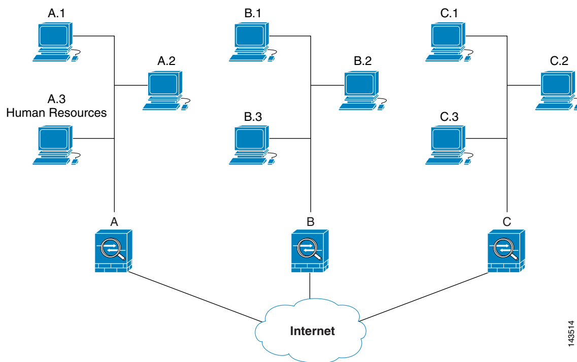
Figure 29-1 Effect of Permit and Deny ACEs on Traffic (Conceptual Addresses)
