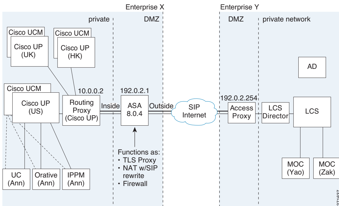
Figure 27-12 Typical Cisco Unified Presence/LCS Federation Scenario
