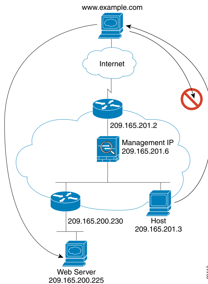
Figure 17-7 Typical Transparent Firewall Data Path
