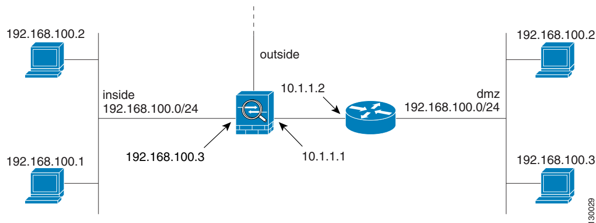
Figure 19-28 Using Outside NAT with Overlapping Networks
