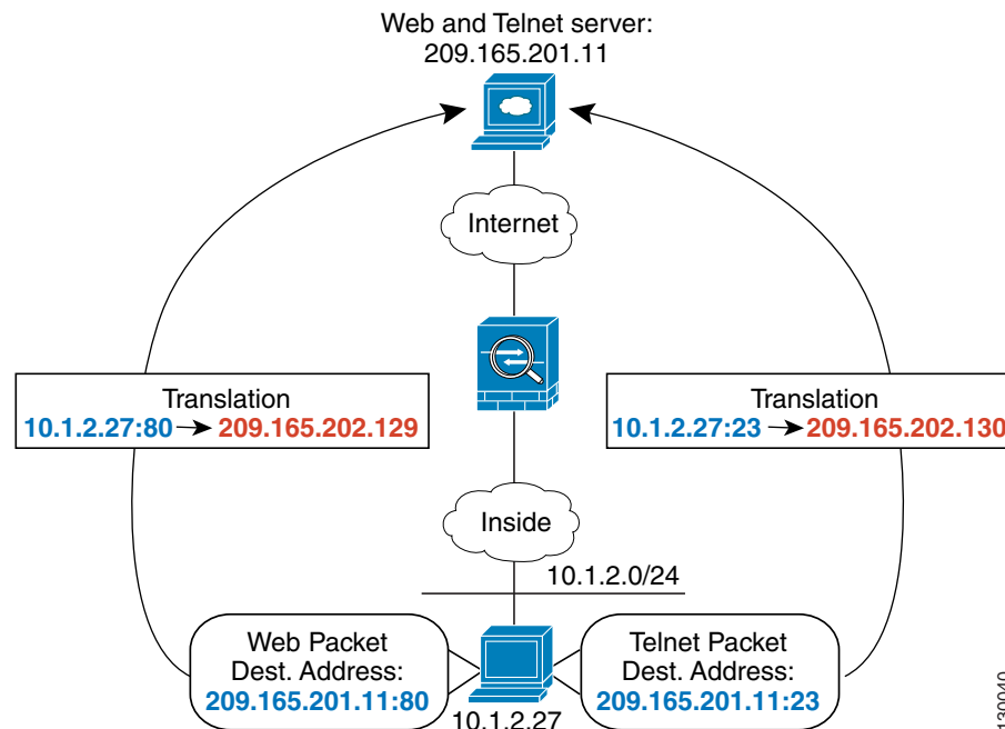
Figure 19-10 Policy NAT with Different Destination Ports
