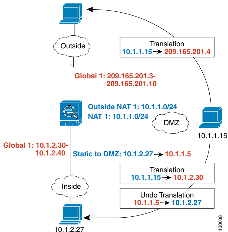
Figure 19-20 Outside NAT and Inside NAT Combined
