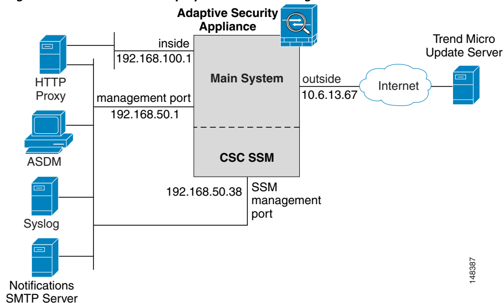
Figure 23-6 CSC SSM Deployment with a Management Network
