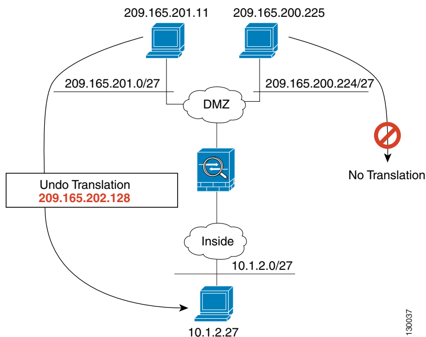
Figure 19-11 Policy Static NAT with Destination Address Translation
