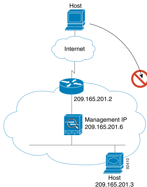
Figure 17-11 Outside to Inside
