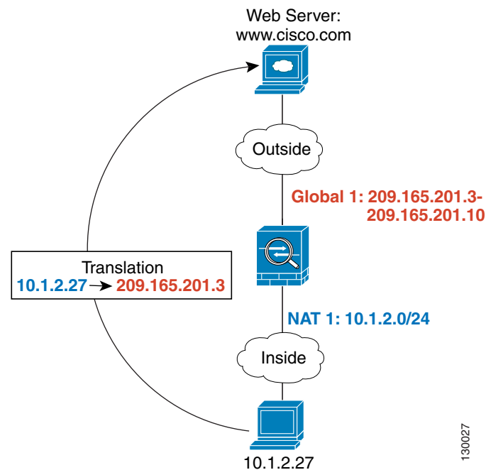
Figure 19-15 nat and global ID Matching
