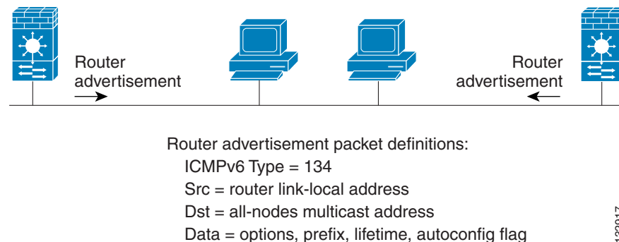
Figure 13-2 IPv6 Neighbor Discovery—Router Advertisement Message
