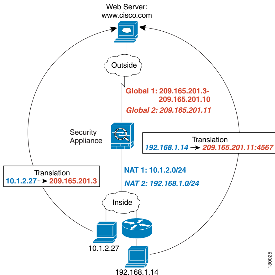
Figure 19-18 Different NAT IDs
