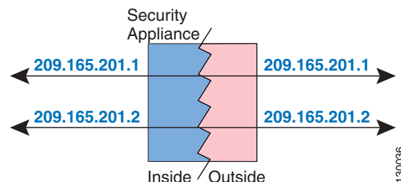
Figure 19-26 Static Identity NAT
