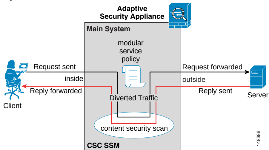
Figure 23-5 Flow of Scanned Traffic with CSC SSM
