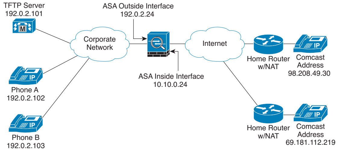
Figure 27-19 LSC Provisioning in Mixed-mode Cisco UCM cluster; Cisco UCM and TFTP Server on Publisher
