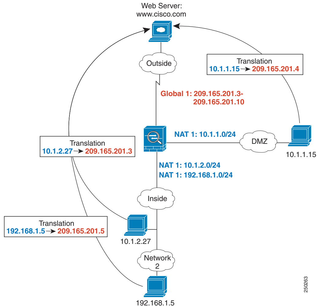
Figure 19-16 nat Commands on Multiple Interfaces
