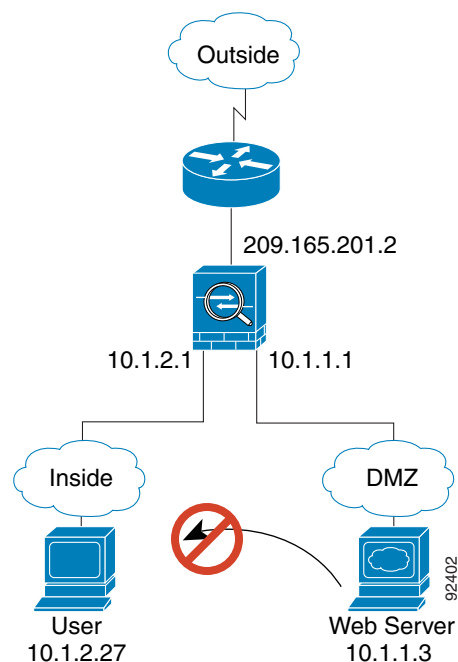
Figure 17-5 DMZ to Inside
