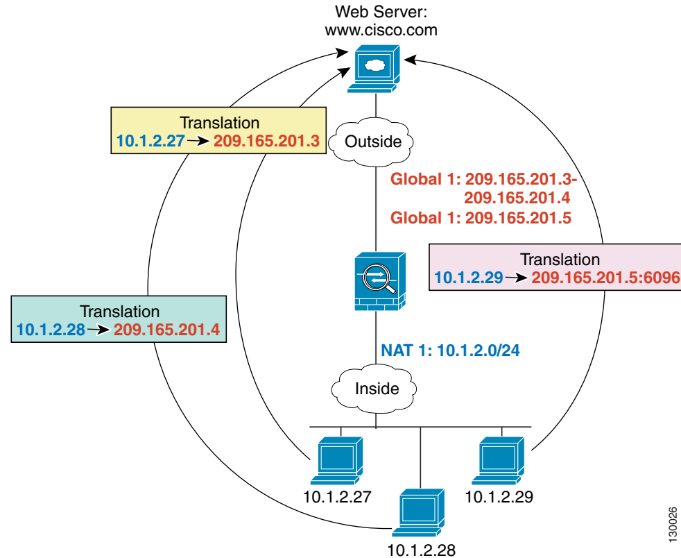
Figure 19-19 NAT and PAT Together
