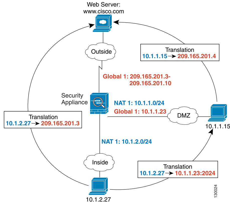
Figure 19-17 global and nat Commands on Multiple Interfaces
