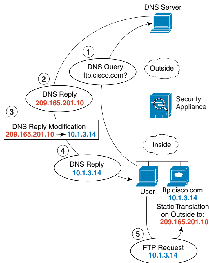
Figure 19-13 DNS Reply Modification
