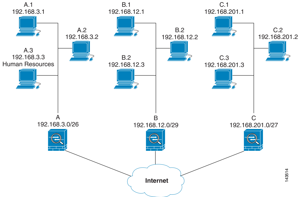
Figure 29-3 Effect of Permit and Deny ACEs on Traffic (Real Addresses)
