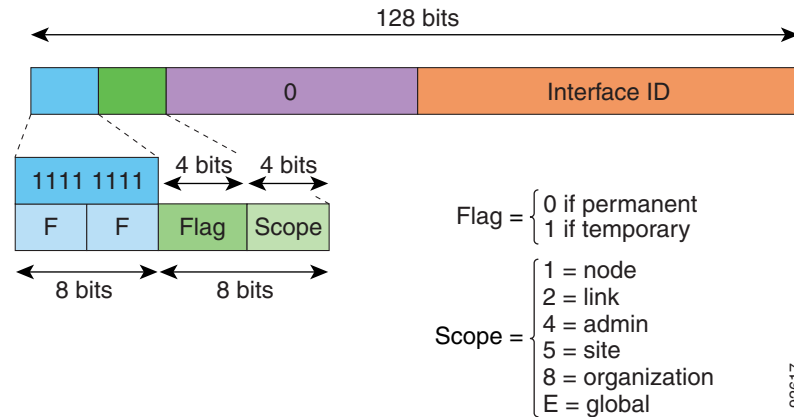
Figure C-1 IPv6 Multicast Address Format
