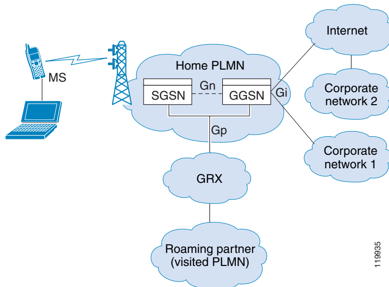
Figure 26-3 GPRS Tunneling Protocol
