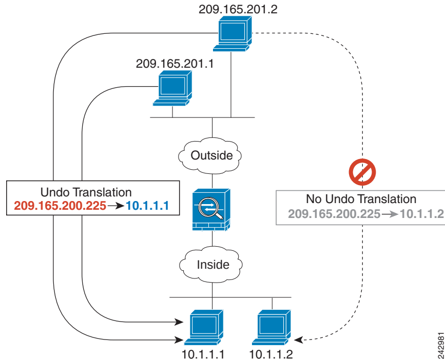
Figure 19-12 Real Addresses Cannot Share the Same Mapped Address
