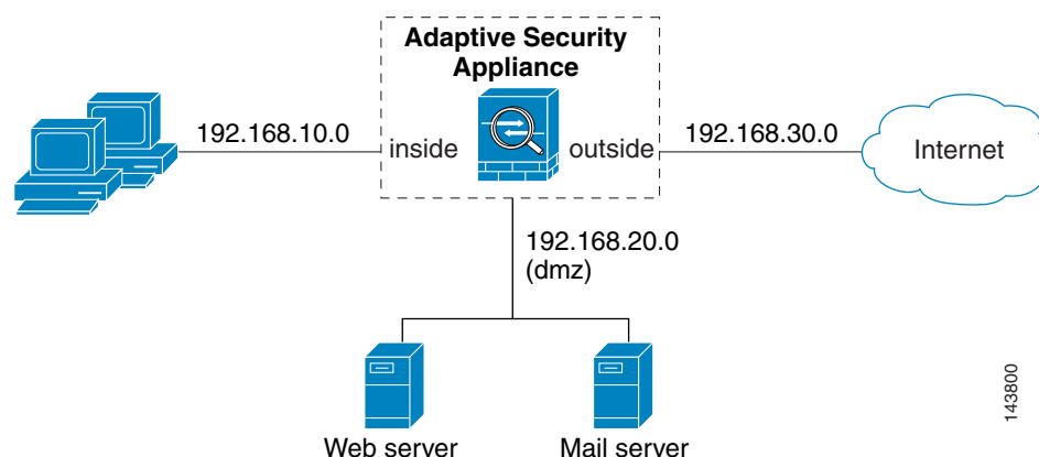
Figure 23-7 Common Network Configuration for CSC SSM Scanning
