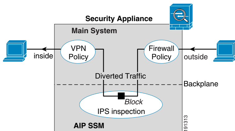
Figure 23-1 AIP SSM Traffic Flow in the Adaptive Security Appliance: Inline Mode
