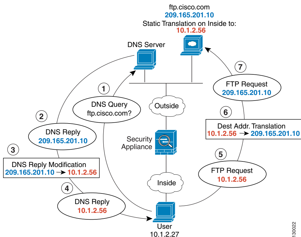
Figure 19-14 DNS Reply Modification Using Outside NAT
