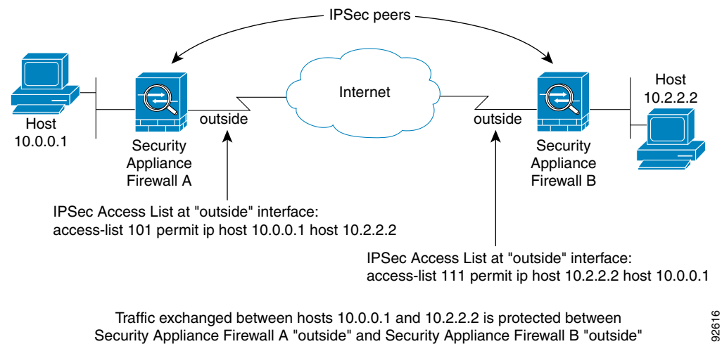
Figure 27-4 How Crypto Access Lists Apply to IPsec
