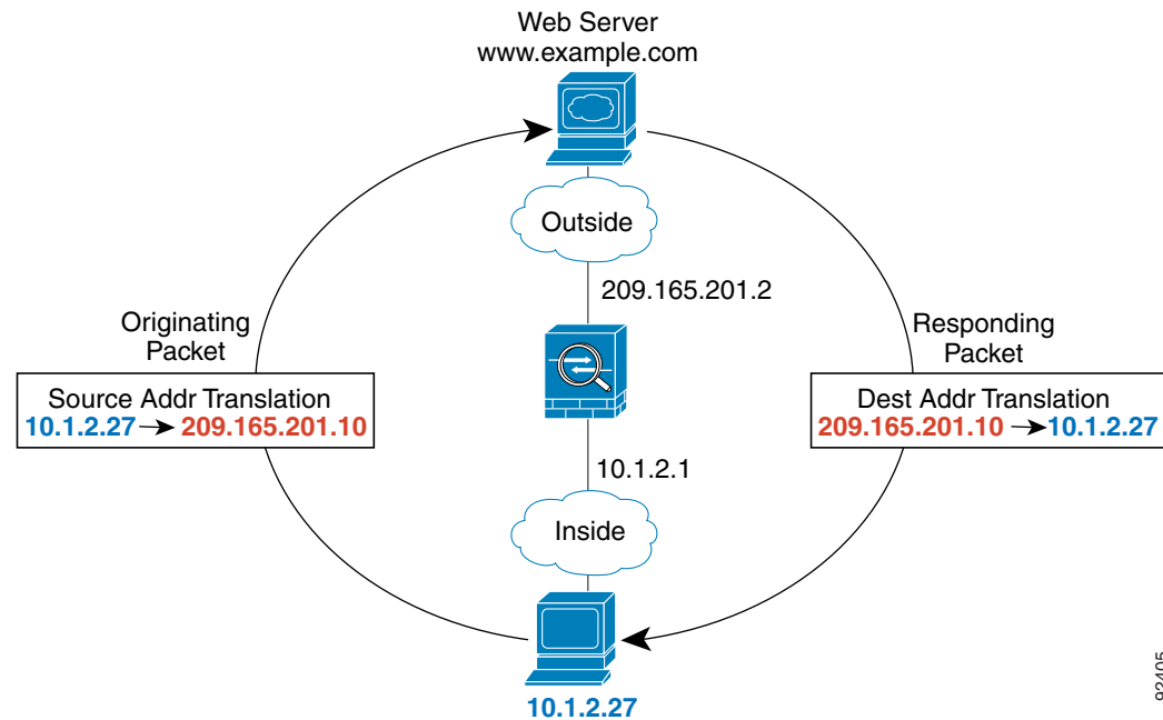
Figure 12-1 NAT Example
