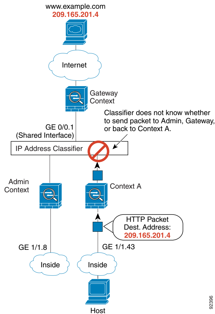
Figure 3-5 Cascading Contexts
