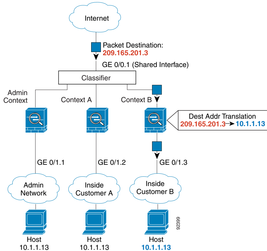
Figure 3-1 Packet Classification with a Shared Interface
