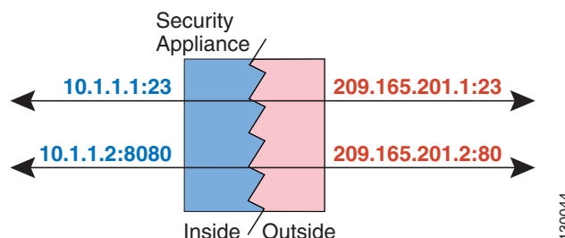
Figure 14-23 Static PAT
