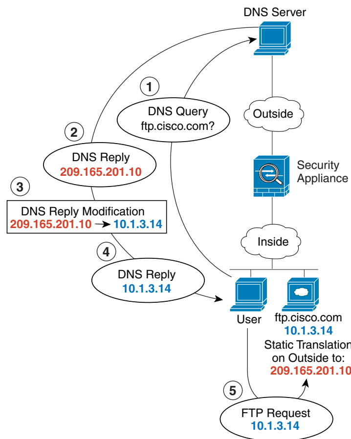
Figure 14-12 DNS Reply Modification
