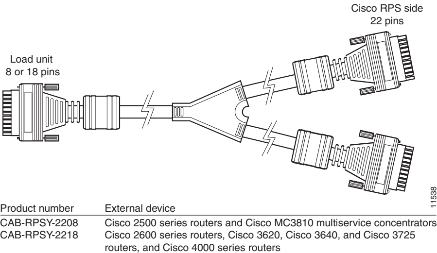
Figure 3-1 Two-to-One Y-Shaped Cable
