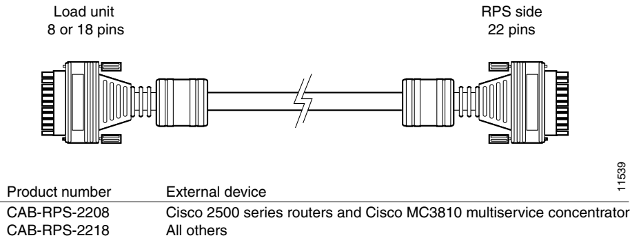
Figure 3-2 One-to-One Cable
