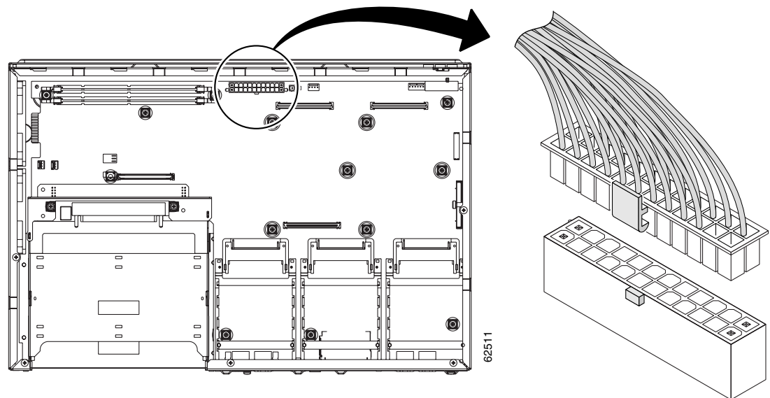
Figure 5 Removing the Cisco 2691 Power Connector
