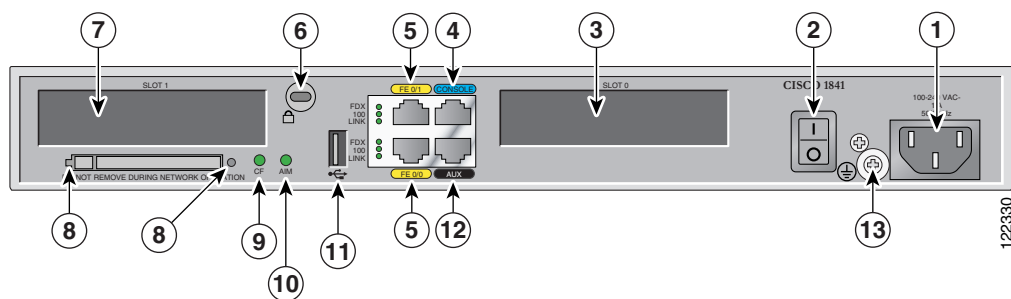
Figure 4 Back Panel of the Cisco 1841 Router
