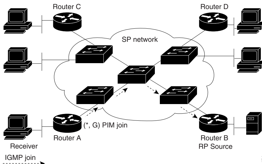
Figure 34-2 PIM Join Message Flow with PIM Snooping
