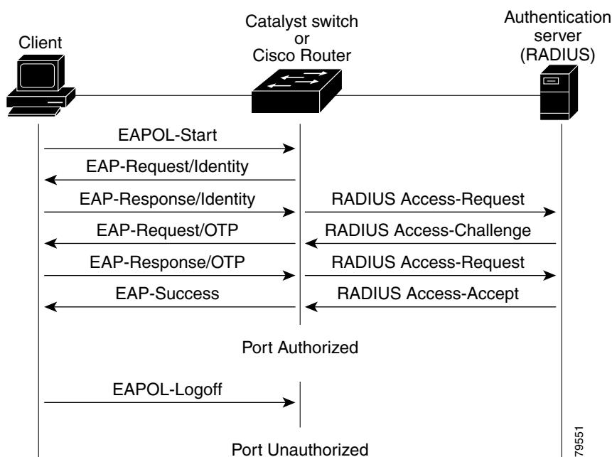
Figure 52-2 Message Exchange
