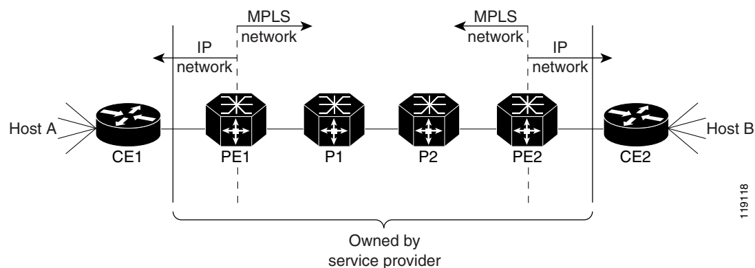
Figure 26-1 MPLS Network
