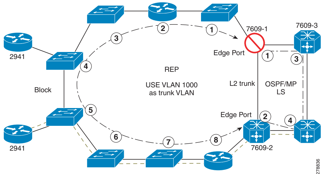
Figure 62-2 Node Failure
