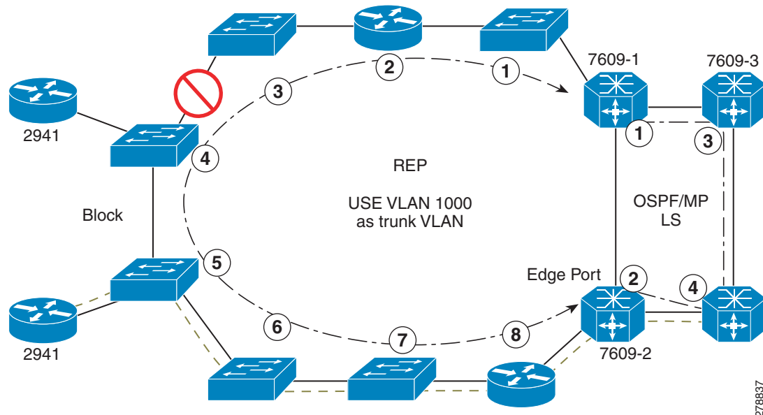
Figure 62-3 Link Failure
