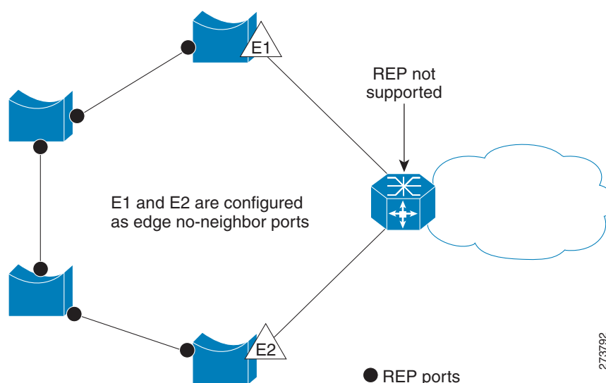
Figure 67-1 Edge No-Neighbor Ports
