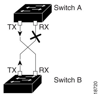
Figure 55-1 Unidirectional Link
