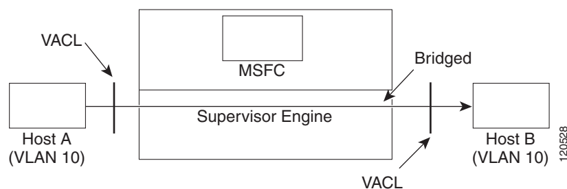
Figure 35-1 Applying VACLs on Bridged Packets
